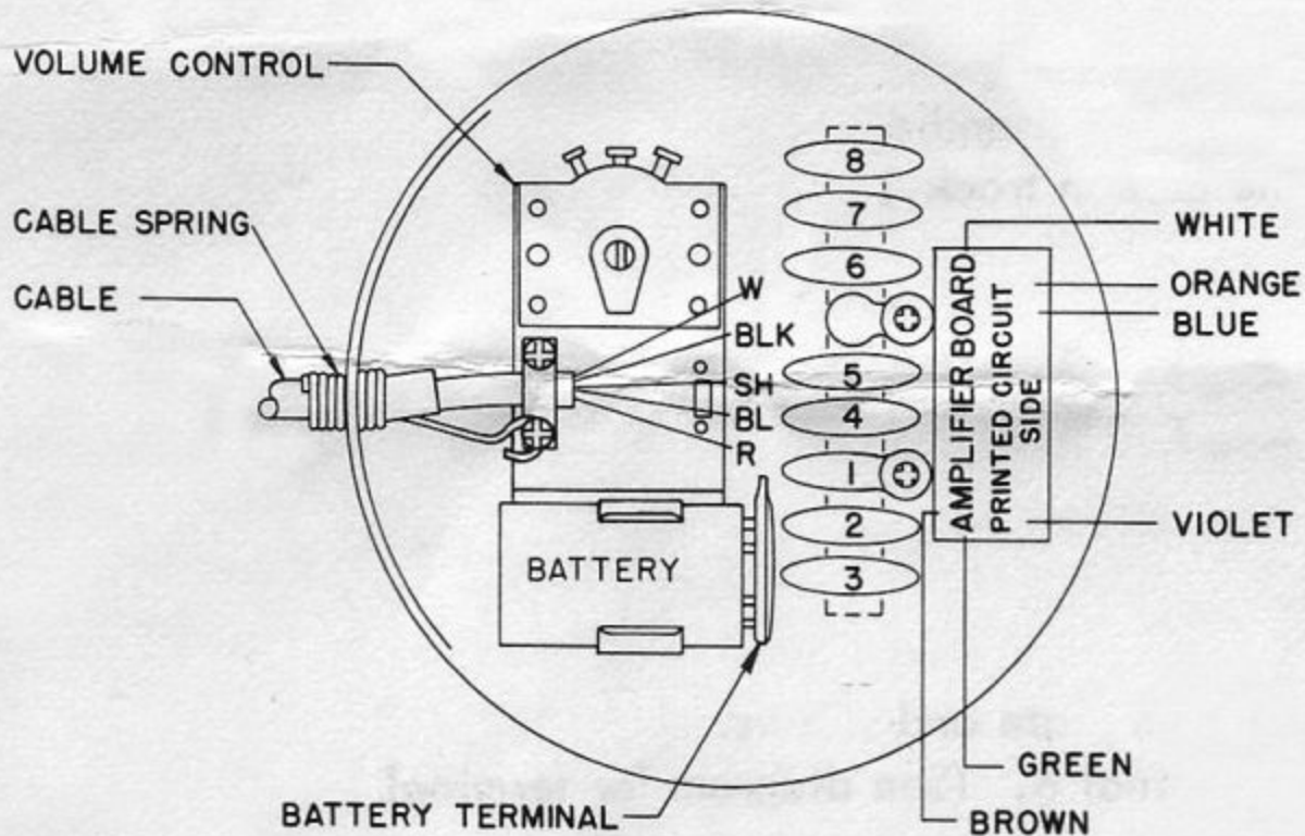
RELATIVE LOCATION OF COMPONENTS IN UG8 BASE
