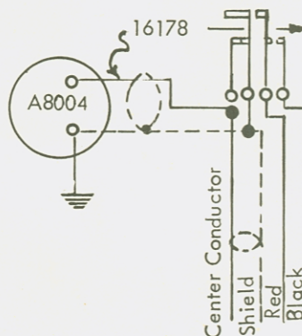
Figure 2 — Model 727SR Wiring Diagram
