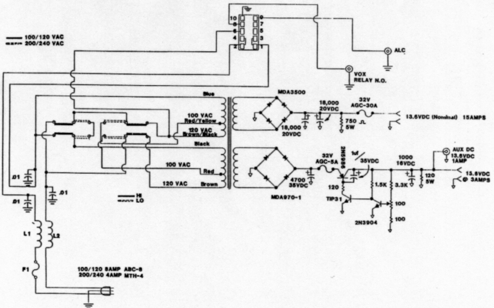
PS75 Schematic Diagram
