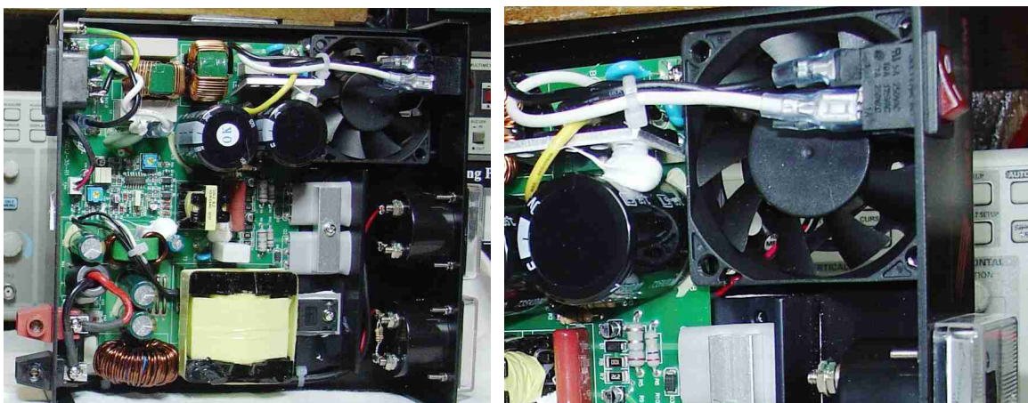
Photo C: Internal view of the SEC-1235M Photo D: Close-up of cooling fan
