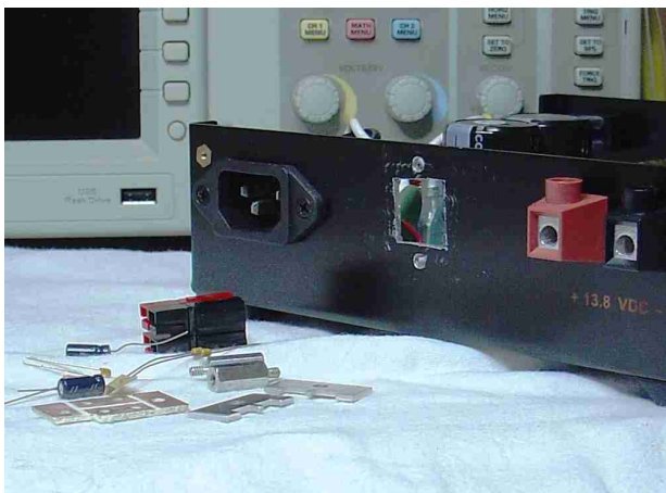
Photo I: Parts and back panel cut-out
