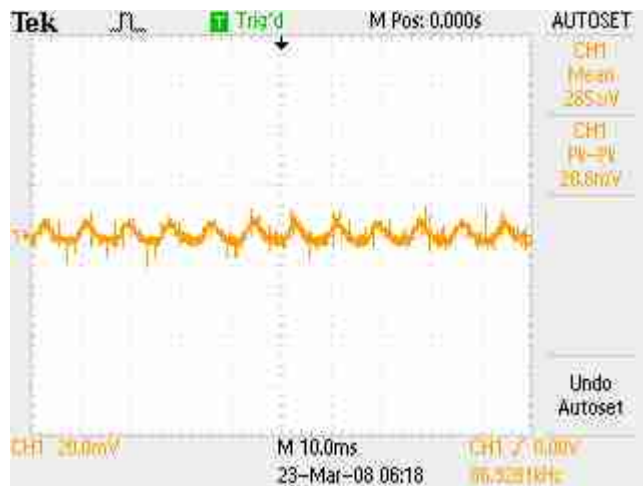
Photo H: Ripple and noise at 24-amp current drain
