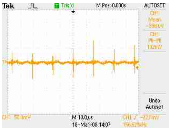
Photo E: No load ripple and noise
