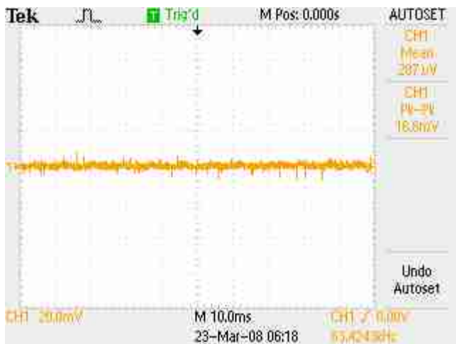
Photo G: Ripple and noise at 3-amp current drain
