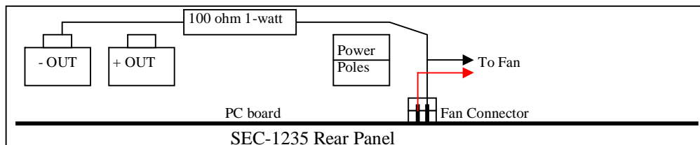
Figure 1: Fan modification
