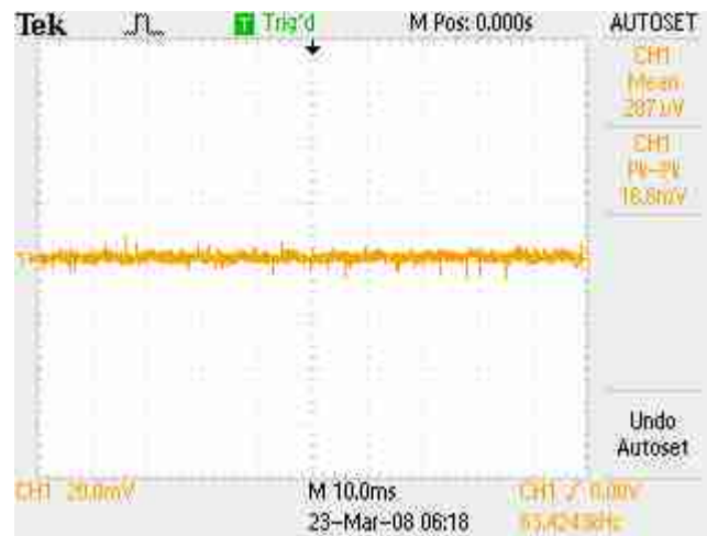
Photo F: Ripple and noise at 1-amp current drain
