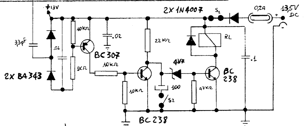
SCHEMA PNB/200 (NOTES 1W2 DBN)
