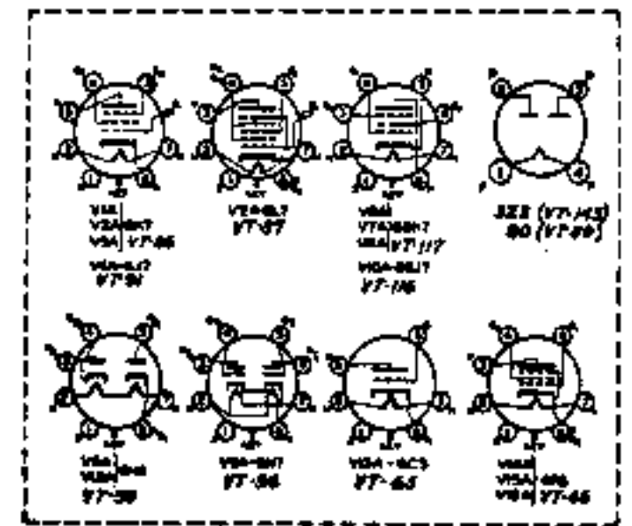
Tube socket terminals.
