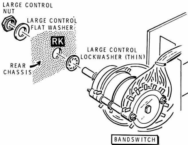
Detail 15-11A
