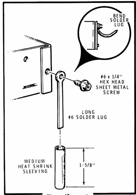
Detail 6-5A
