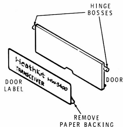
Detail 15-3C
