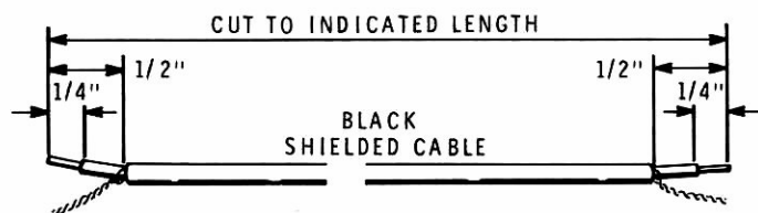
Detail 10-11A
