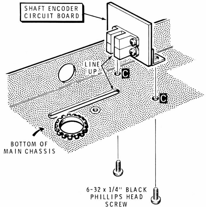
Detail 15-2D
