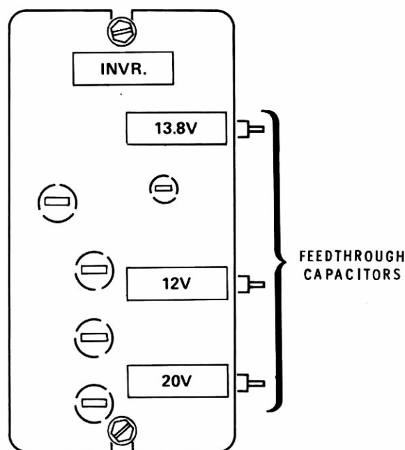
Detail 7-8A
