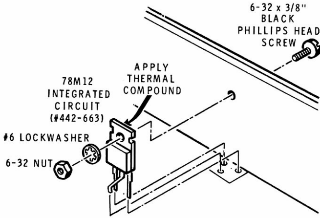
Detail 7-5C
