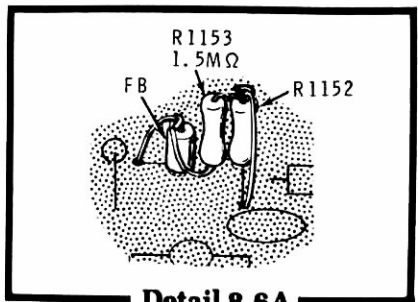
Detail 8-6A
