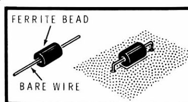
Detail 8-1A
