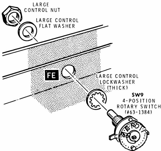
Detail 15-4B
