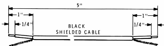
Detail 15-8C
