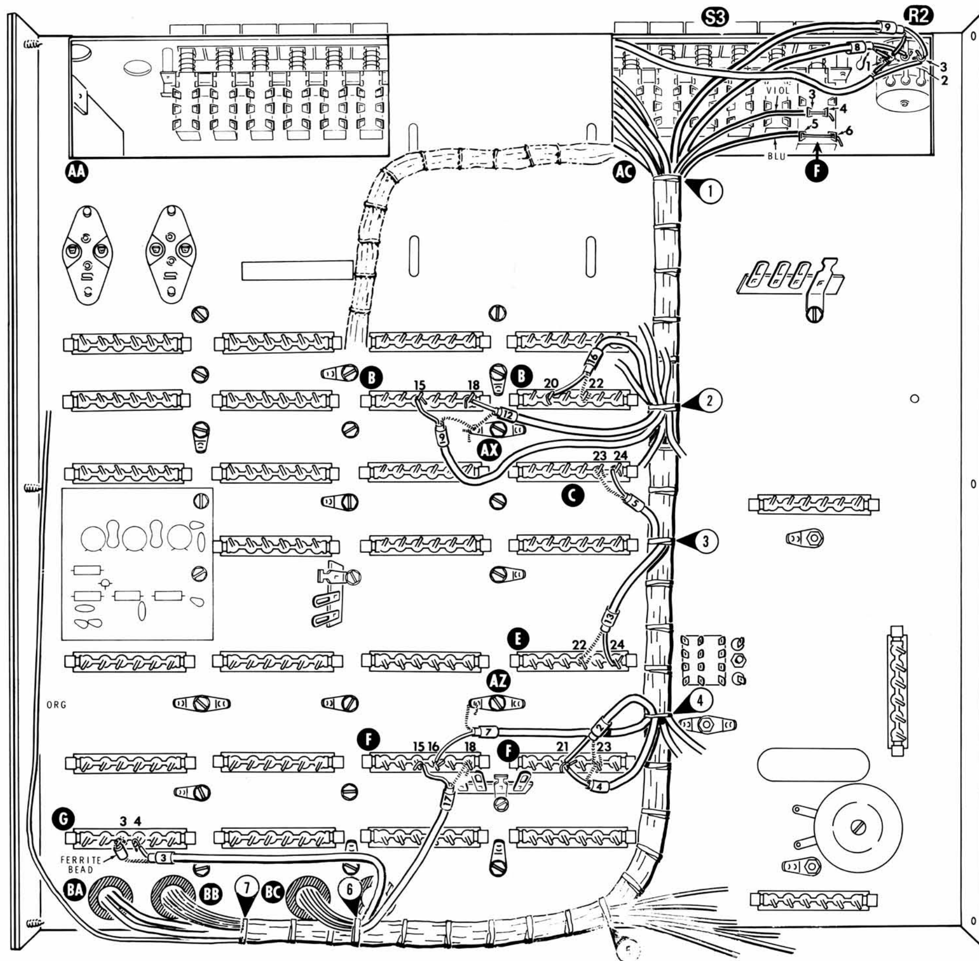
PICTORIAL 12-21
