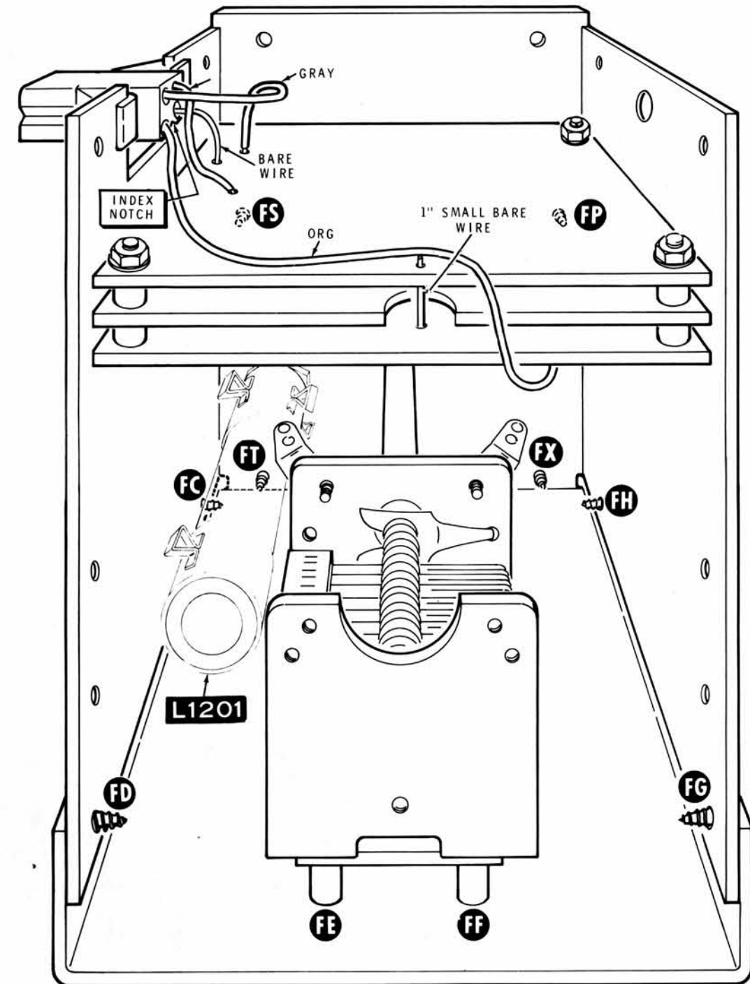
PICTORIAL 1-12
