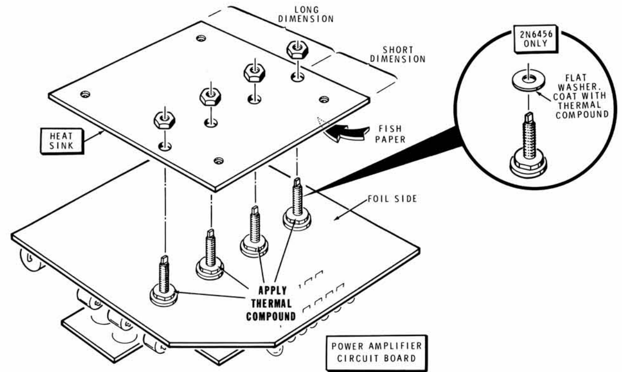
PICTORIAL 11-11
