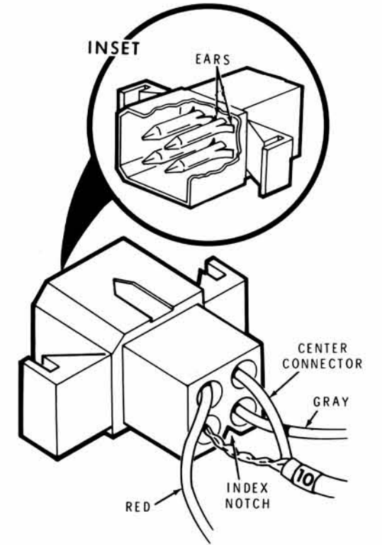
Detail 12-29B
