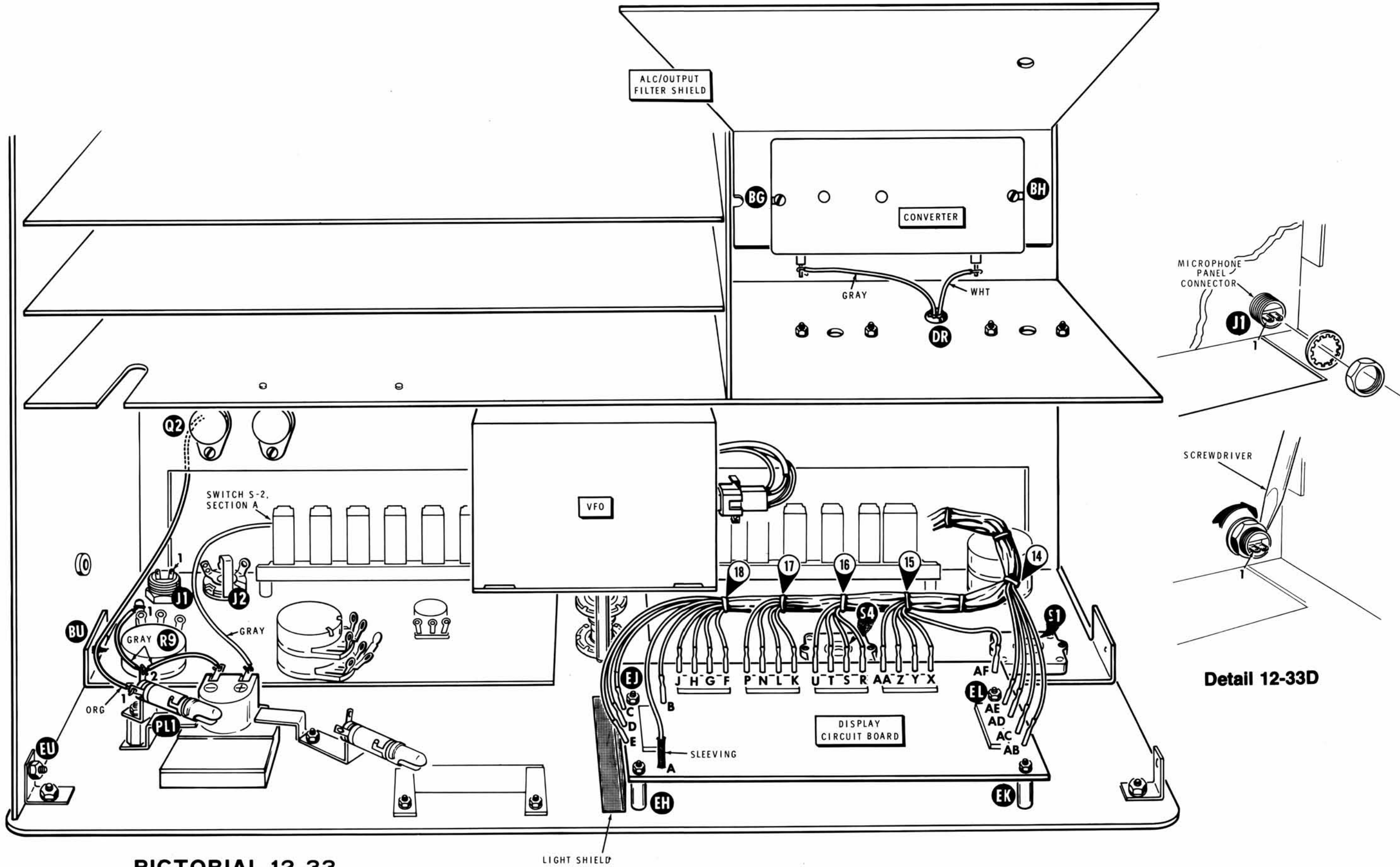
PICTORIAL 12-33
