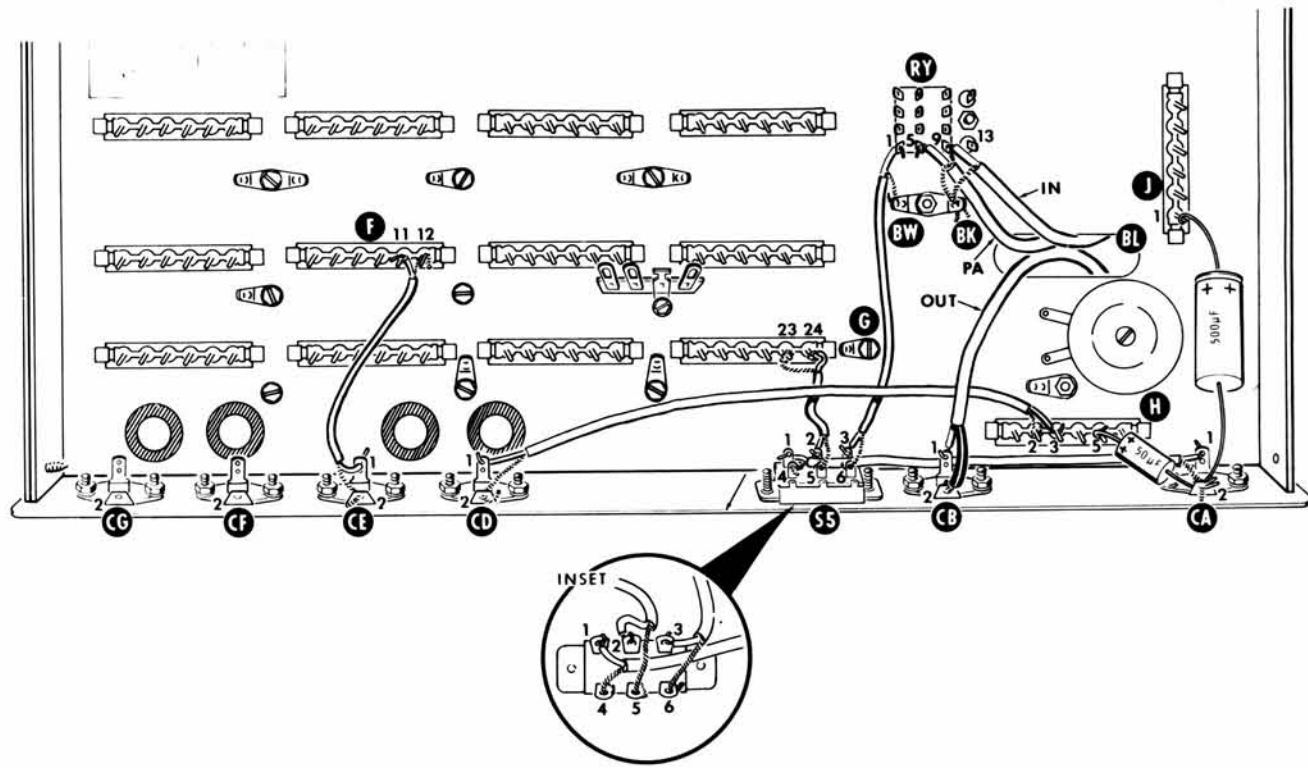
PICTORIAL 12-28
