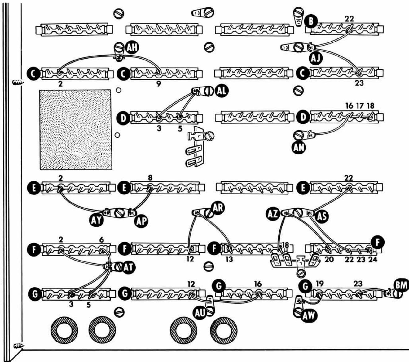
PICTORIAL 12-4
