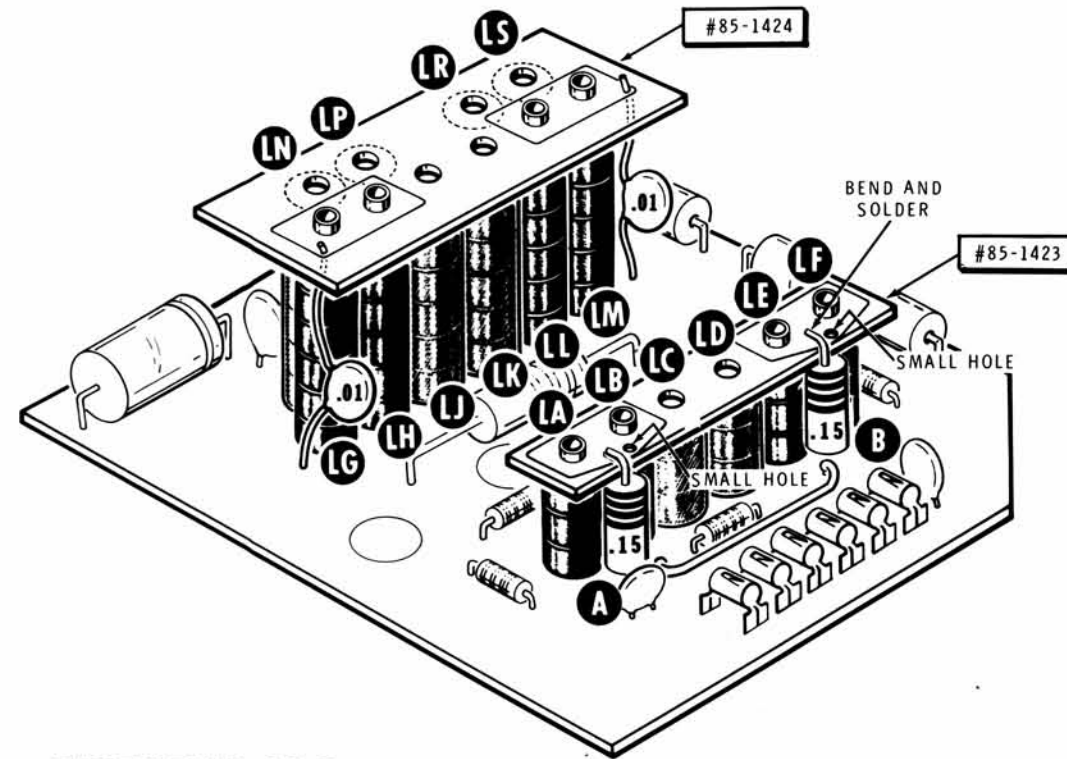
PICTORIAL 11-5
