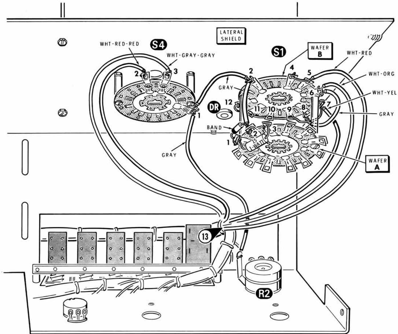
PICTORIAL 12-30
