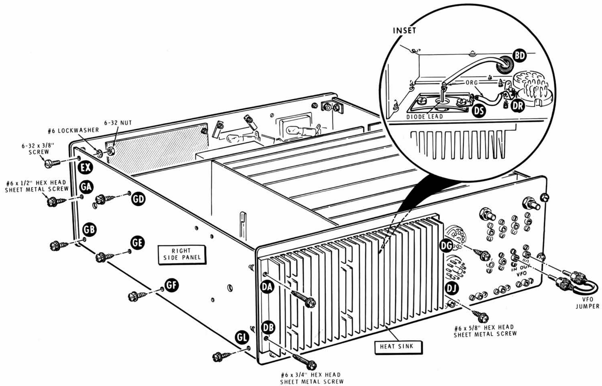
PICTORIAL 12-34
