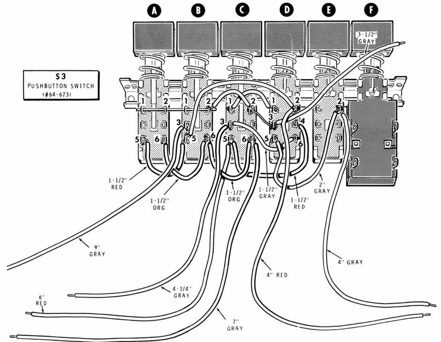
PICTORIAL 12-8
