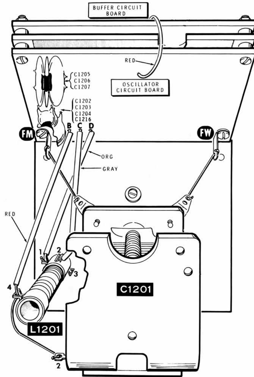
PICTORIAL 1-11
