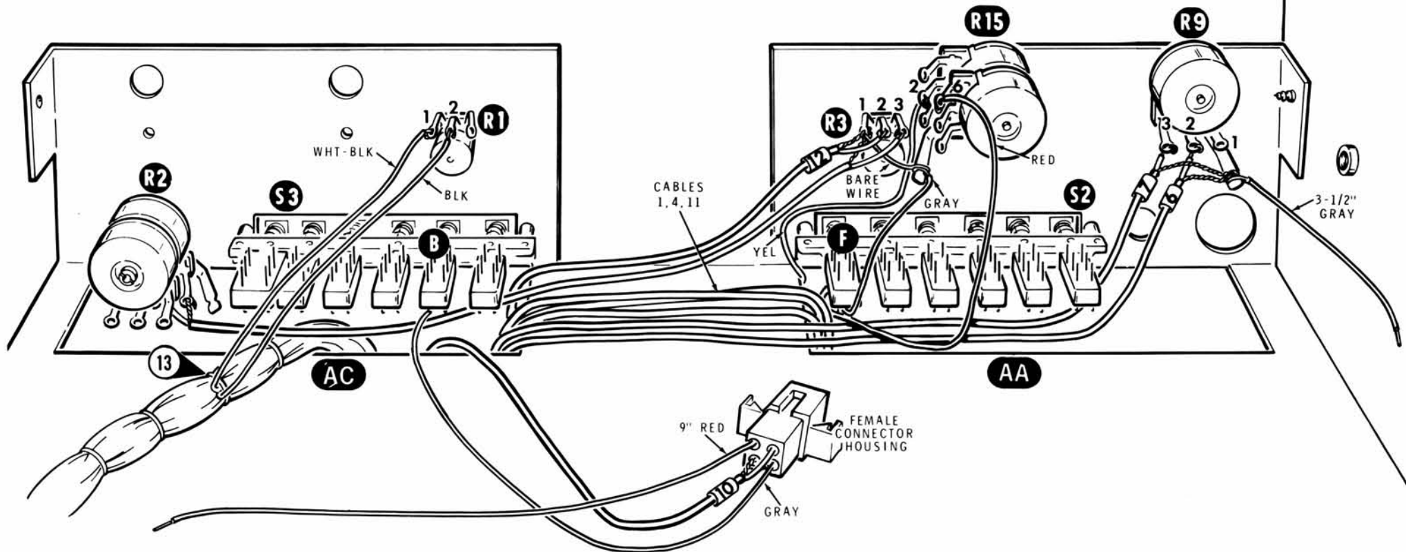
PICTORIAL 12-29
