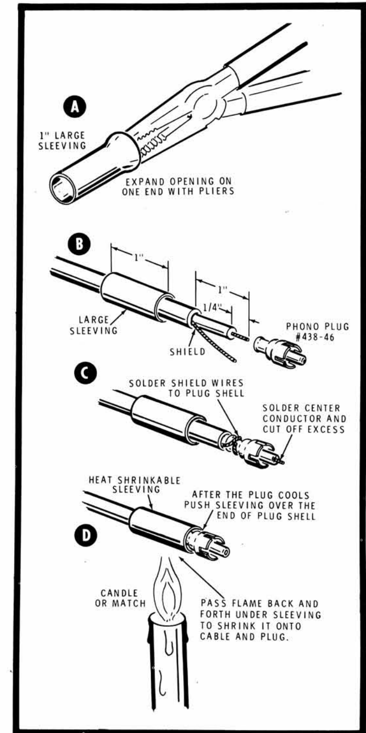
Detail 12-19B
