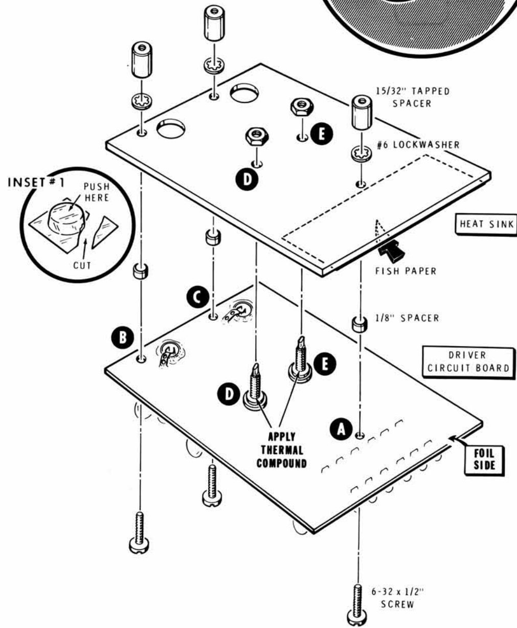
PICTORIAL 6-6
