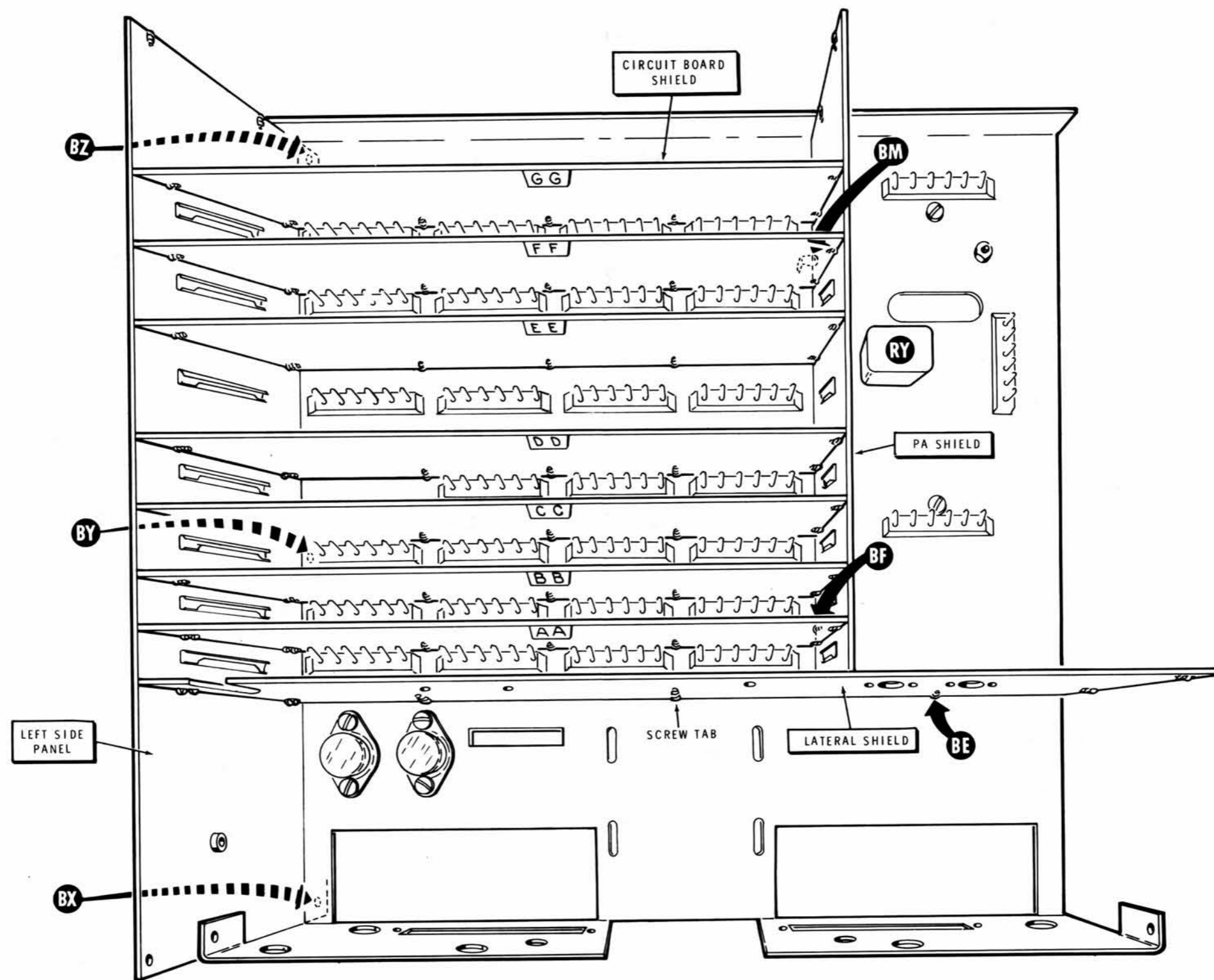
PICTORIAL 12-2
