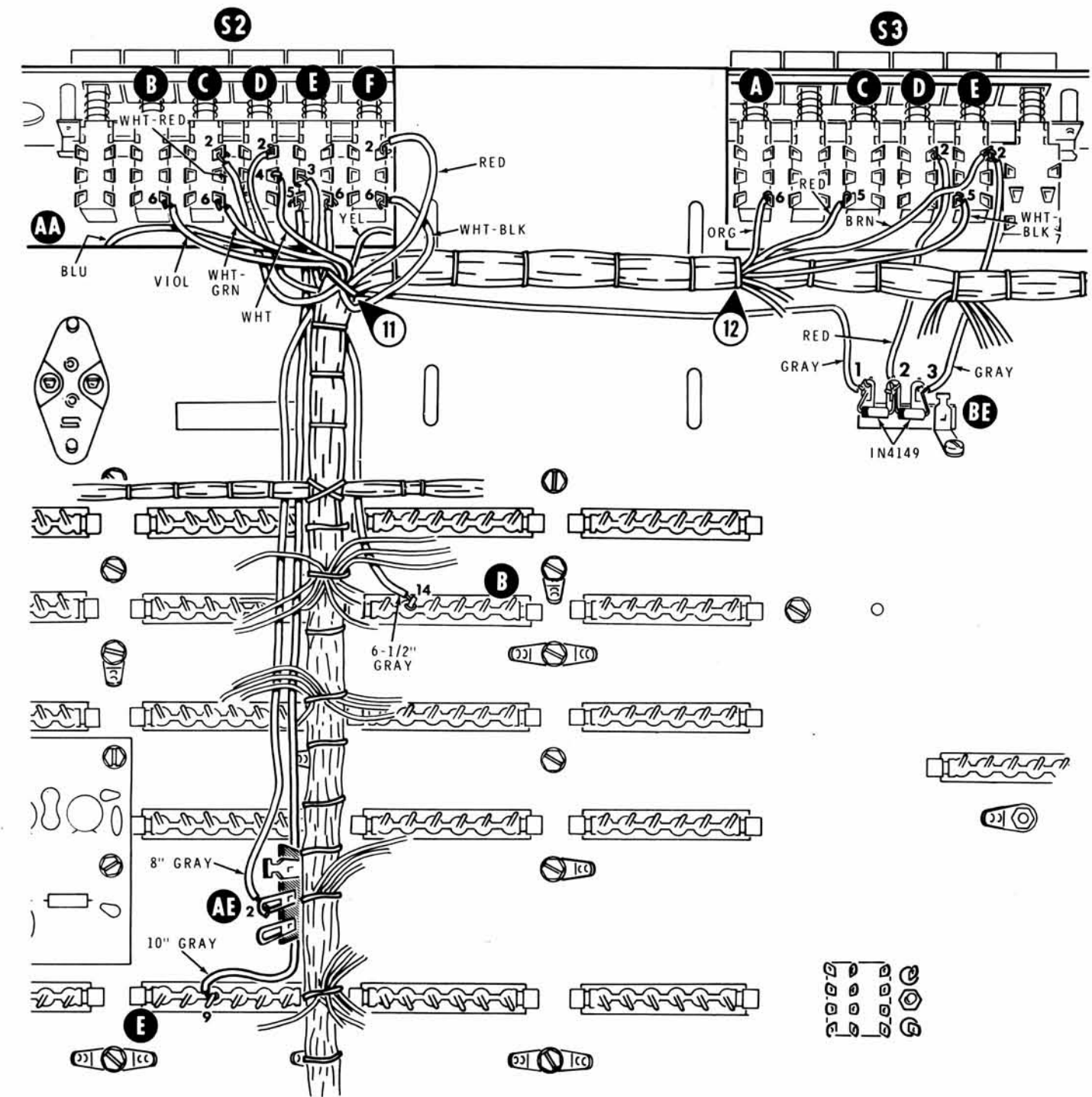
PICTORIAL 12-13
