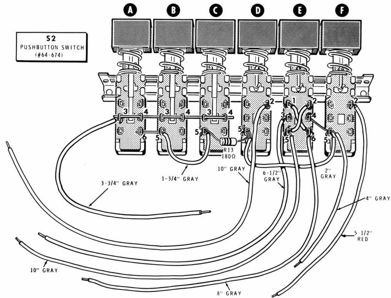
PICTORIAL 12-9
