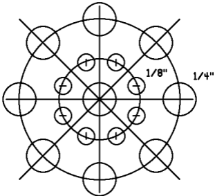
SPEAKER DRILL HOLE PATTERN
