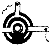
CATHODE BACK VIEW OF JACK
