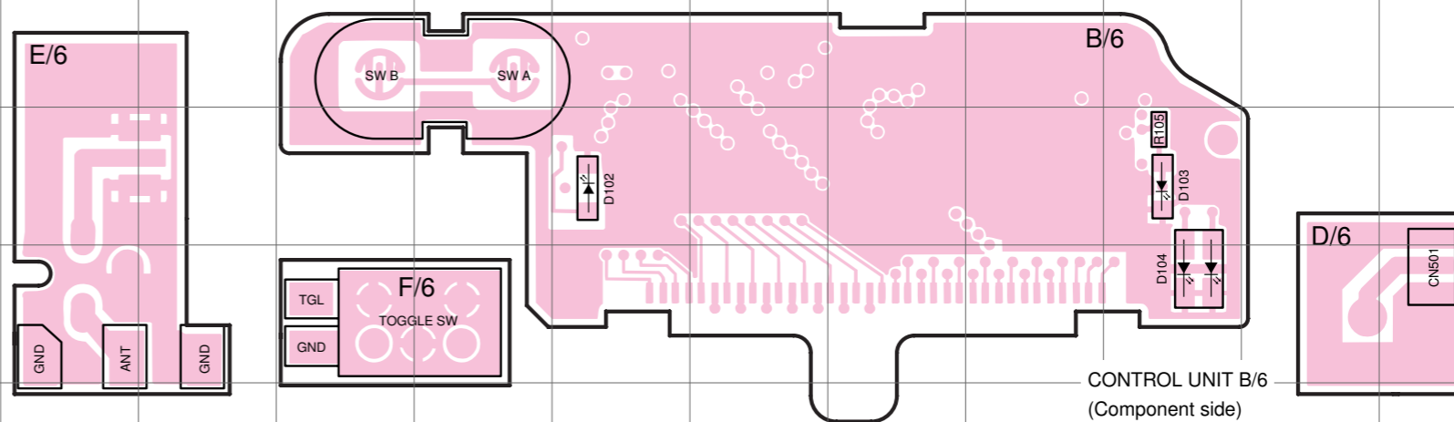
CONTROL UNIT (X53-3930-10 B/6,D/6,E/6,F/6) Component Side View
