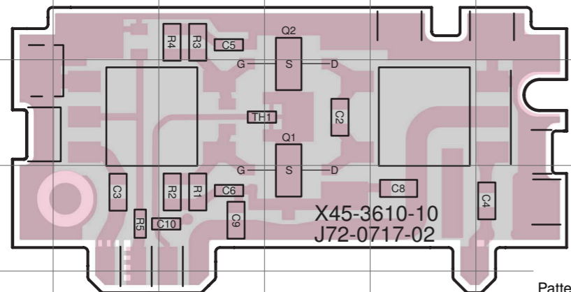
FINAL UNIT (Component side)
