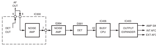
Fig. 4 Squelch circuit
