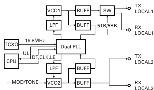
Fig. 7 PLL block diagram
