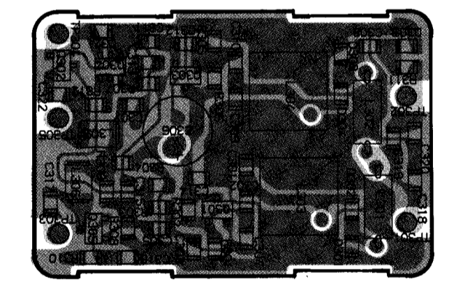
Obverse View of "Mixed Component" Side
