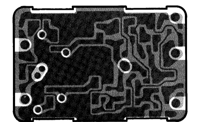
Obverse View of Solder Side
