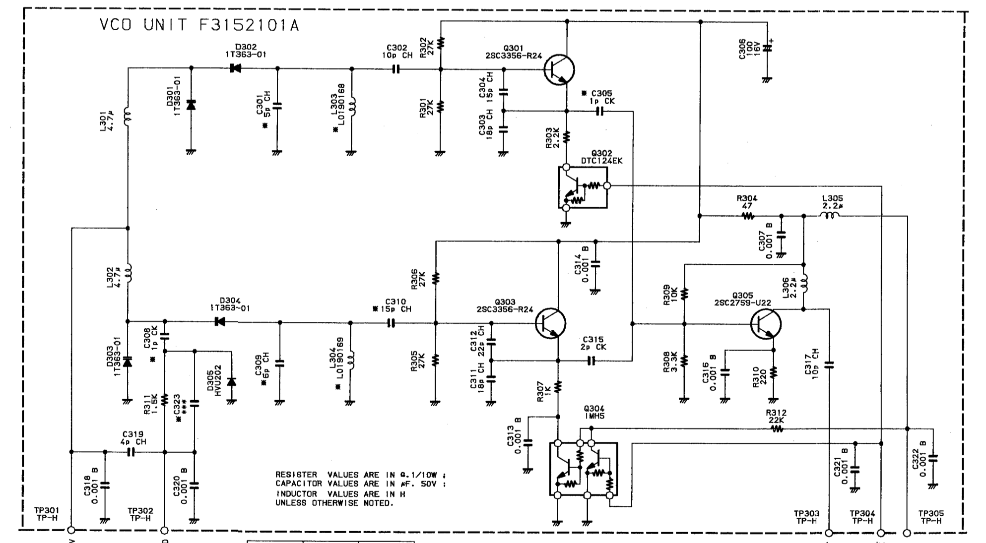
Obverse View of "Mixed Component" Side
