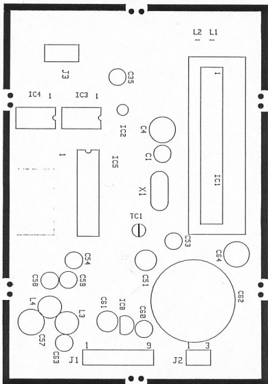
PLL UNIT COMPONENT LOCATION FOR THE AR2002 SERIAL NUMBERS 1500 UP
