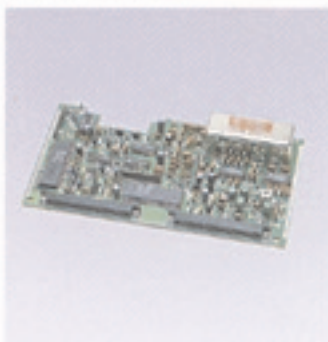
• CFL-243 BWC Unit
