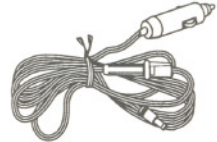
Cigarette Lighter Power Cord Adaptor (PS001)
