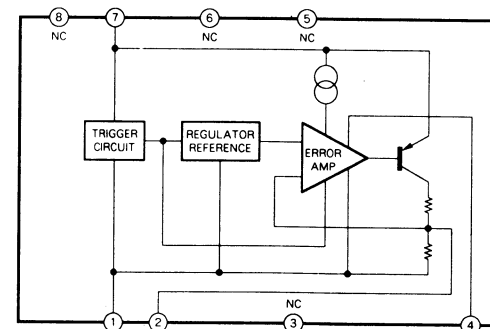
IC203 LA5003M
