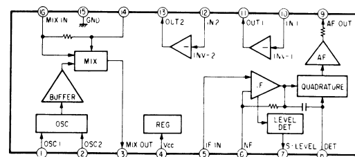
IC1 TA7761F
