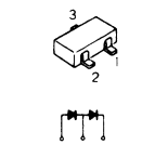
1SS123
