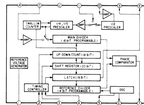
IC202 CXD1118M
