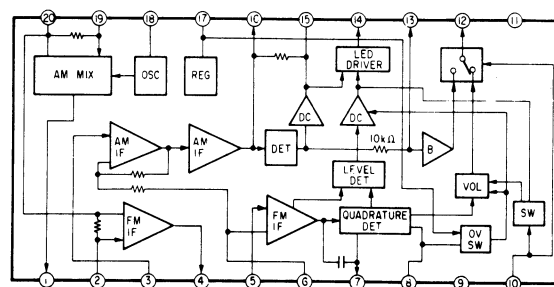
IC2 TA7758P
