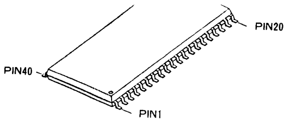
M5M82C055AFP (Q5004, Q5005, Q5006, Q5007)
