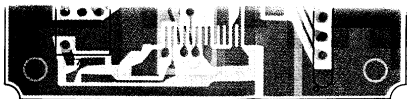
(obverse view of "component" side)
