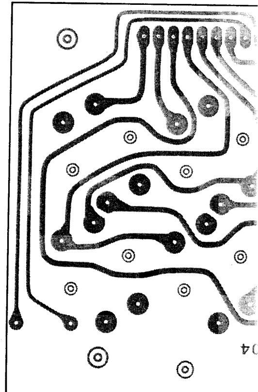
(reverse view of "solder" side)
