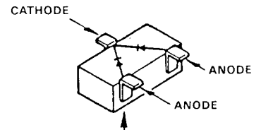
Marked Surface MC2838 (A6) (D5001, D5002, D5003, D5004, D5008, D5009)
