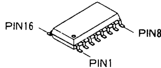
uPD74HC239G (Q5039) MC14028BFL (Q5040, Q5041) TC74HC173AF (Q5011) TC74HC191AF (Q5020, Q5021, Q5022, Q5023, Q5024, Q5025, Q5026, Q5027) TC74HC138F (Q5008, Q5009)
