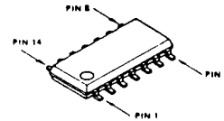
MC14013BFL (Q5028, Q5029) MC14584BFL (Q5036, Q5037, Q5038) MC74HC32FL (Q5010, Q5012) MC74HC00FL (Q5013, Q5014, Q5015) TC4072BF (Q5030, Q5031, Q5032) TC4081BF (Q5033, Q5034, Q5035) TC74HC08AF (Q5055, Q5056, Q5057, Q5058)
