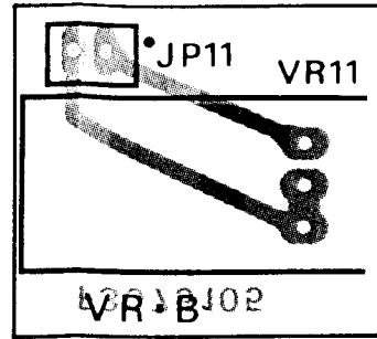
(obverse view of "component" side) (obverse view of "component" side)
