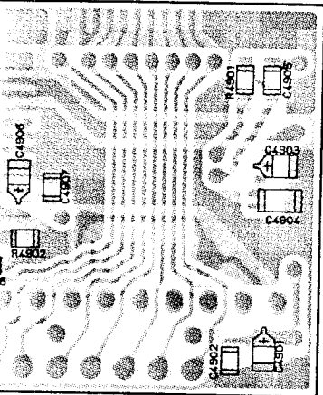
(view of "chip-only" side)
