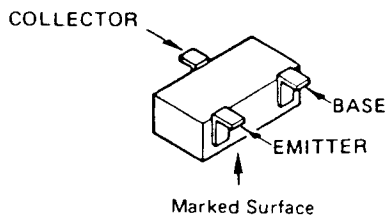
Marked Surface 2SC1623(L6) (Q7701, Q7704, Q7801, Q7804)
