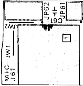
(obverse view of "component" side)
