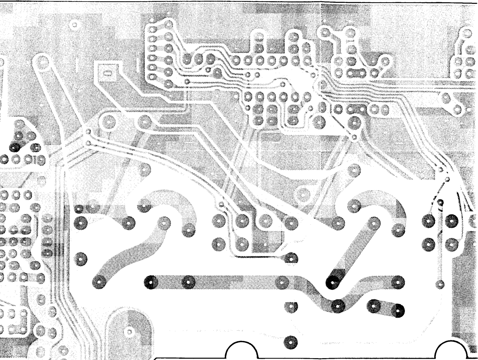
(obverse view of "solde
