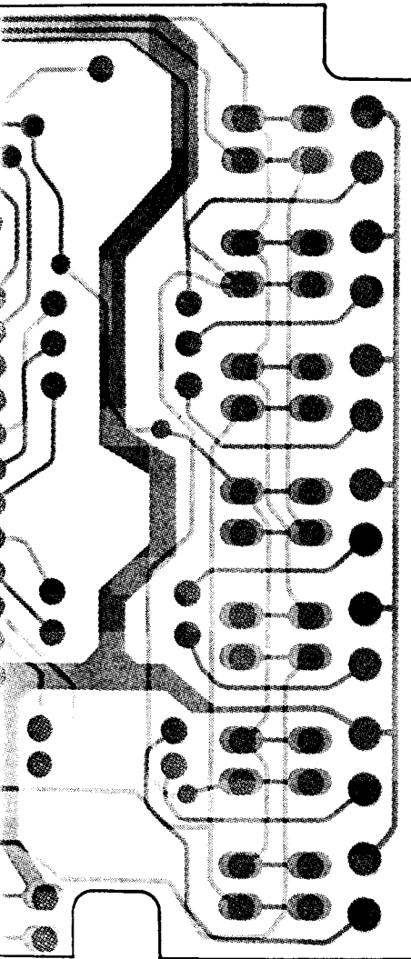
Partial view of "solder" side)
