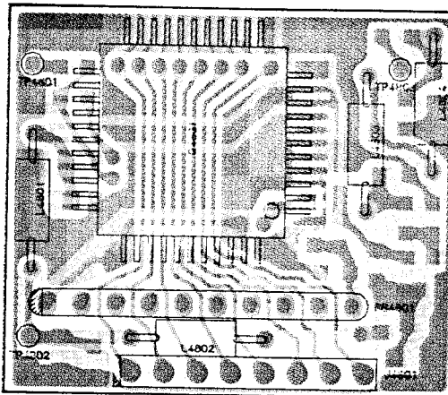
(obverse view of "component" side)
