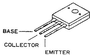
2SC2987Q (Q7601, Q7602, Q7603)
