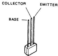
BA1A4P (Q8401, Q8501)
