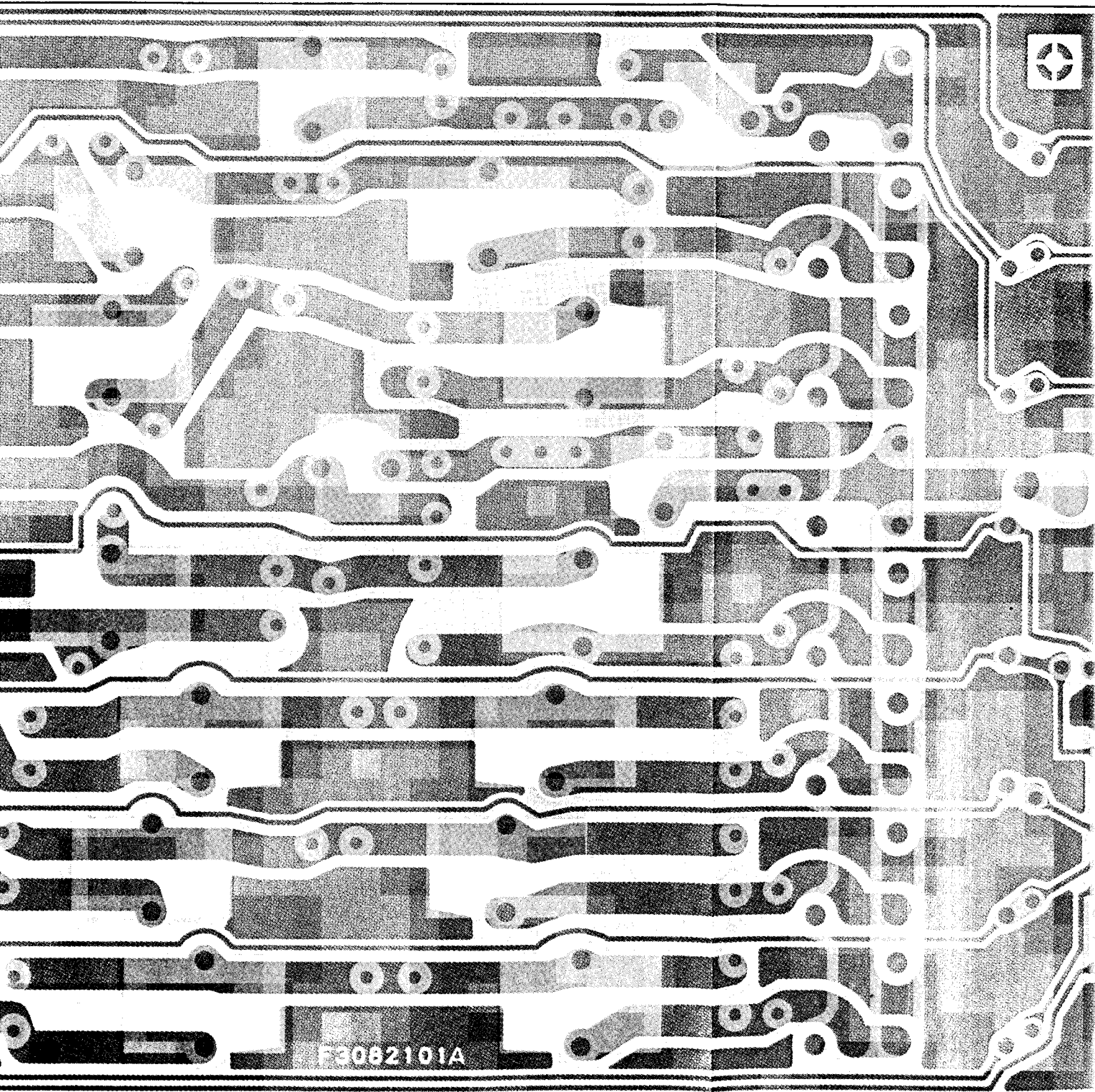
(obverse view of "solder" sic
