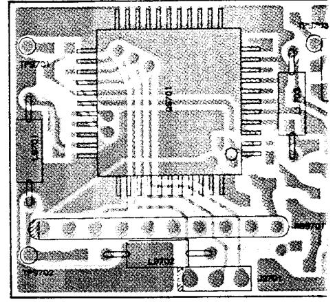
(obverse view of "component" s
