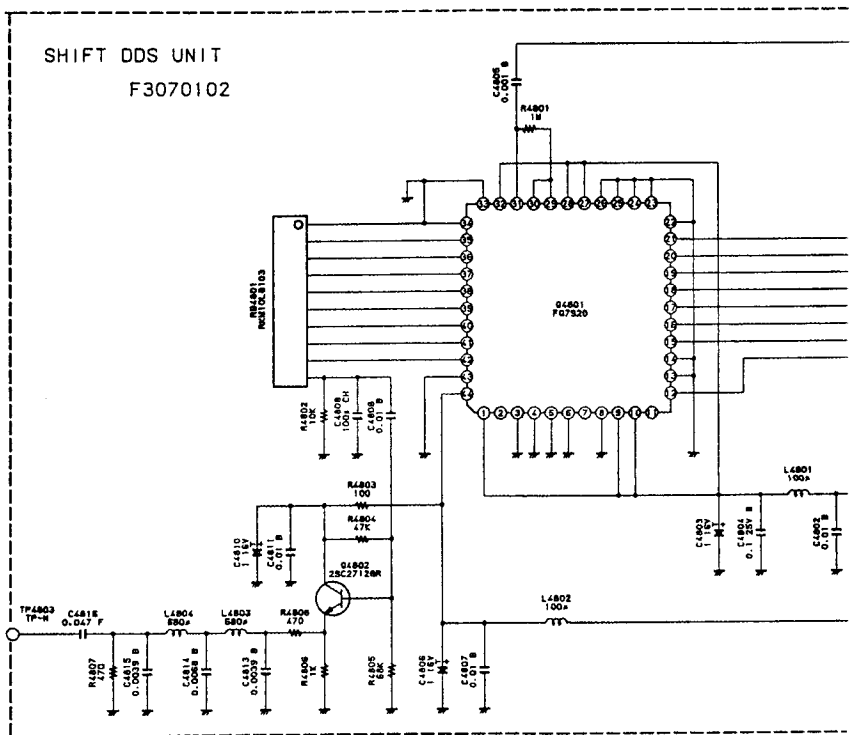
(SHIFT DDS UNIT schern)
