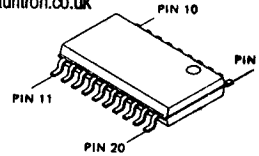
TC74HC541AF (Q5016, Q5017, Q5018, Q5019)
