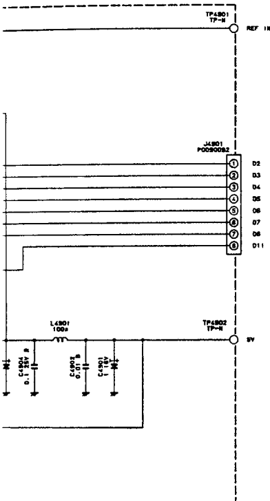
chip-only side schematic diagram)
