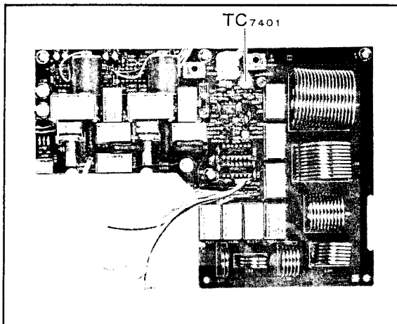
TC7401 Location on Tuner Main Unit
