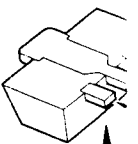
Marked S M51943B (Q5047)
