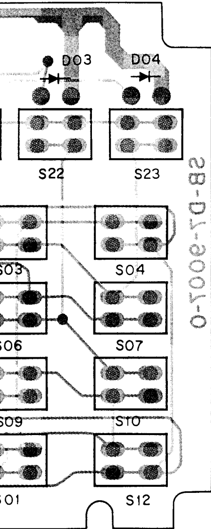
View of "component" side)
