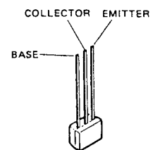
BN1A4P (Q9805, Q9806)
