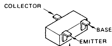
Marked Surface 2SC1623 (L6) (Q7701, Q7704, Q7801, Q7804)
