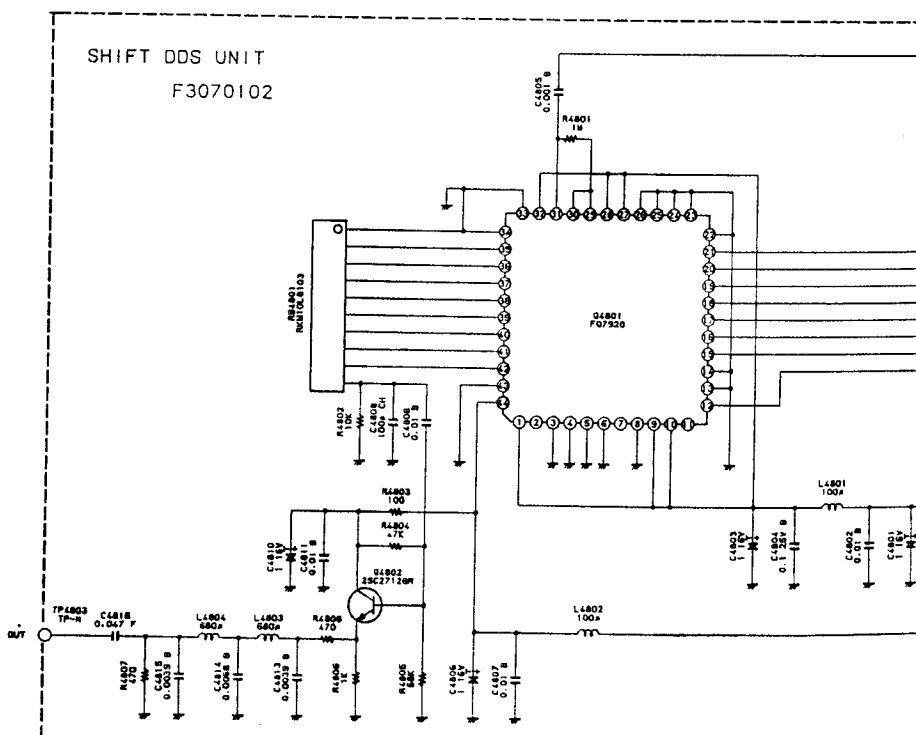
(SHIFT DDS UNIT schematic)
