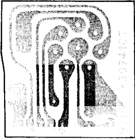
(obverse view of "solder" side)
