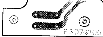
(obverse view of "solder" side)
