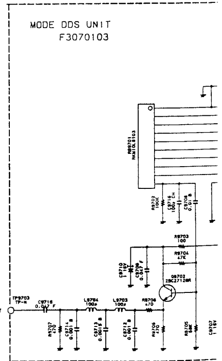
NOTE: RESISTOR VALUES ARE IN A KΩ UNIT
