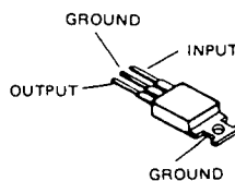
L7809 (Q7618, Q7619)
