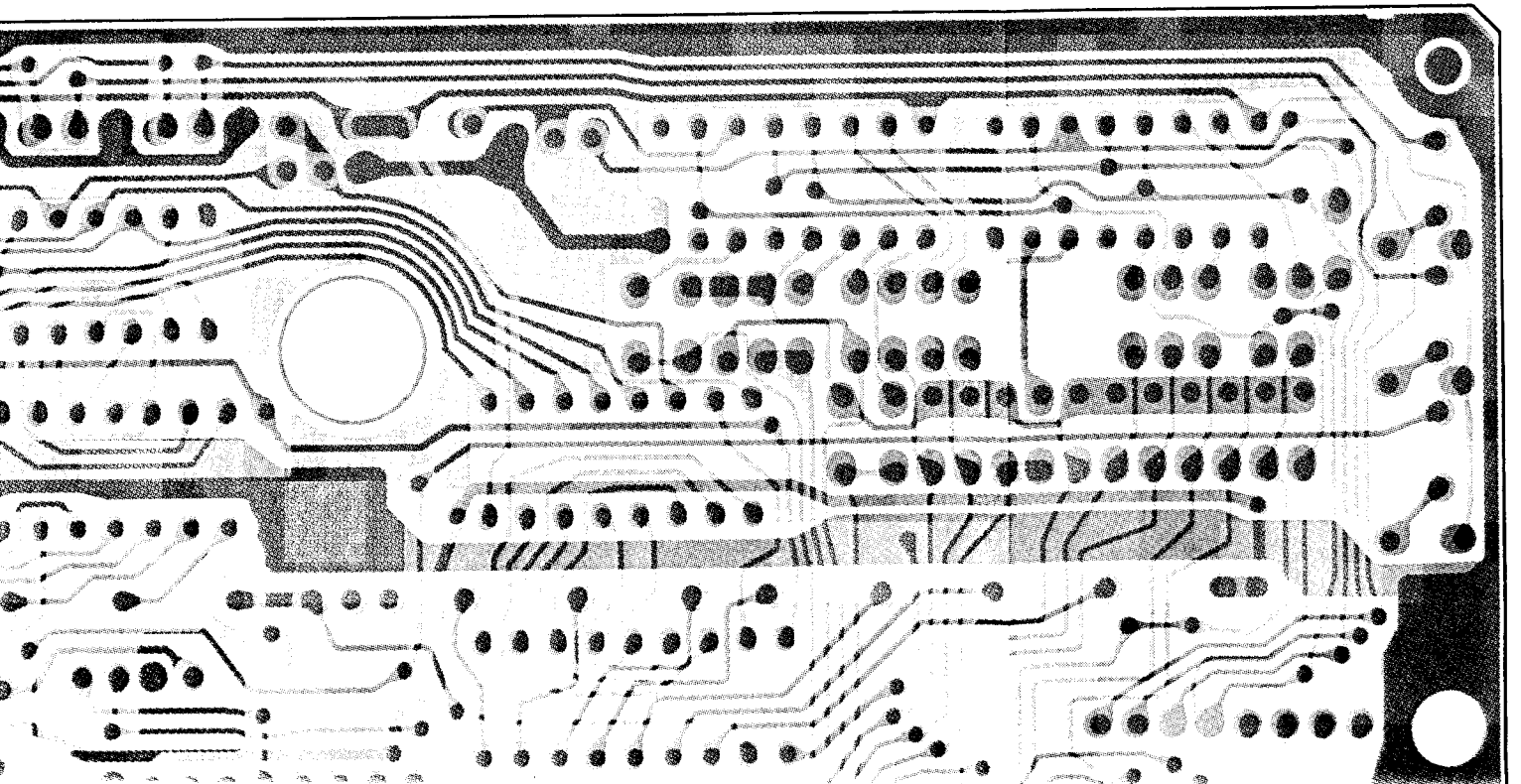
(obverse view of "component" side)
