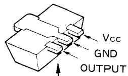
Marked Surface M51943BML (A4) (Q5047)
