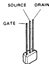
2SK192A-BL (Q4033) 2SK192AGR (Q4050, Q4052, Q4054, Q4056)
