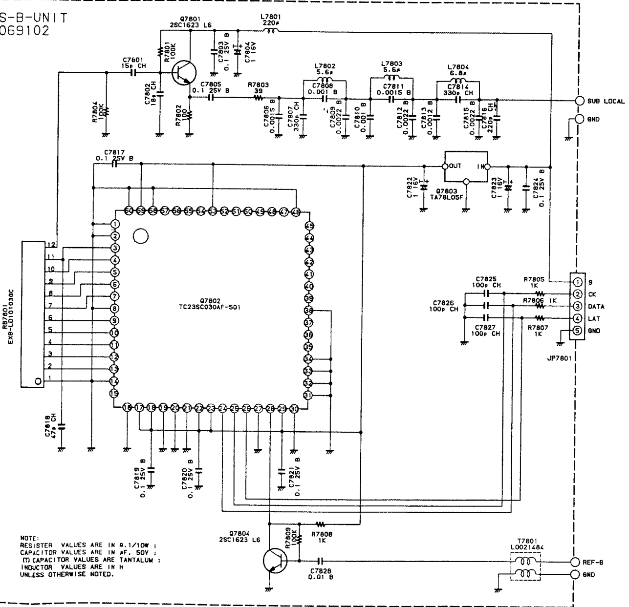
(DDS-B UNIT schematic diagram)
