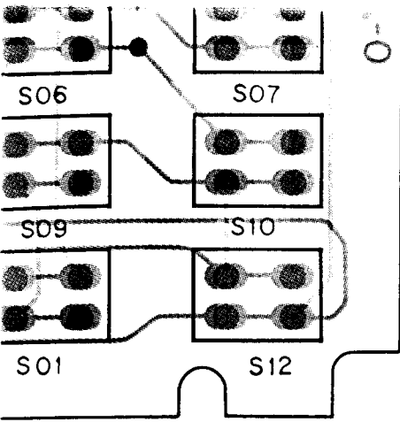
Partial view of "component" side)
