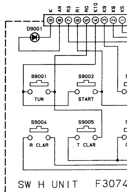
(SW H UNIT schematic
