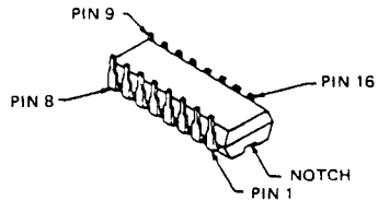
MC14028BCP (Q8009, Q8010) \mu PD74HC238C (Q8006, Q8007, Q8008)
