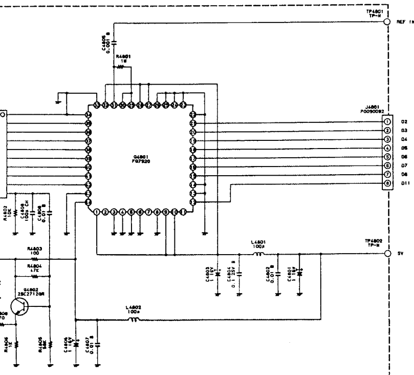
(SHIFT DDS UNIT schematic diagram)
