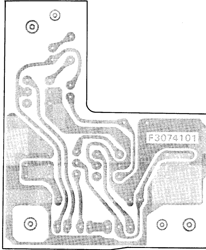
(obverse view of "solder" side)
