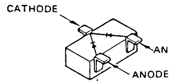
(obverse view of "chip-only")
