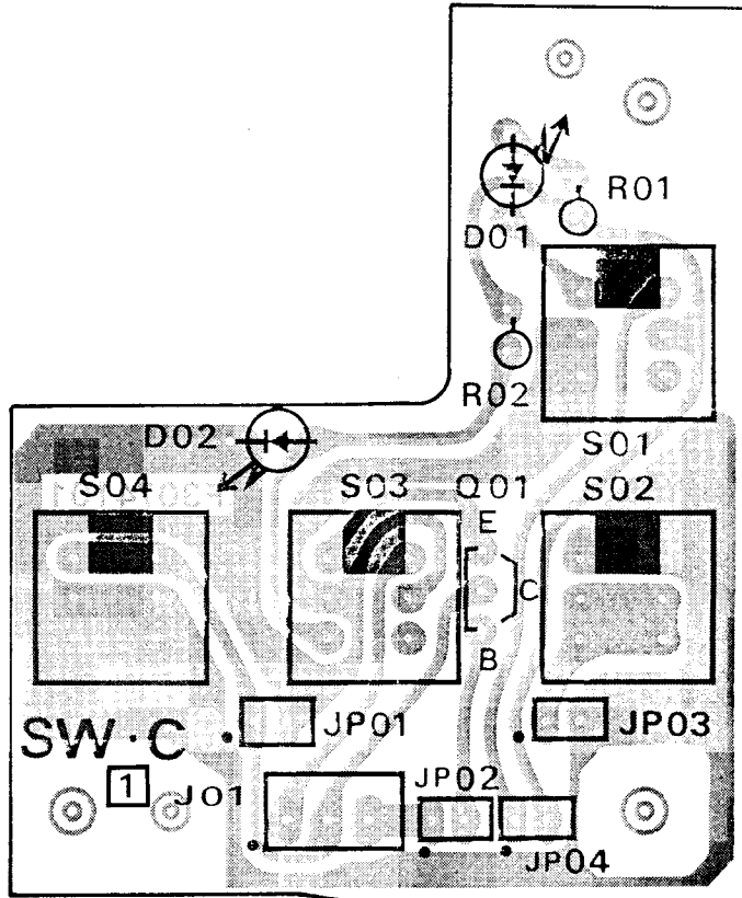
(obverse view of "component" side)
