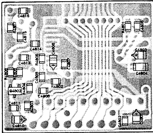
(obverse view of "chip-only" side)
