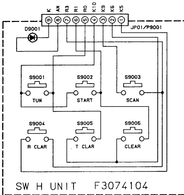
(SW H UNIT schematic diagram)
