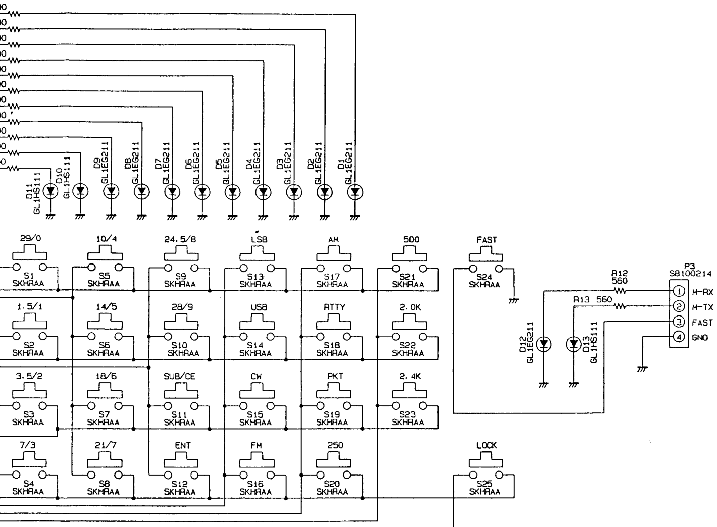
(schematic diagram)
