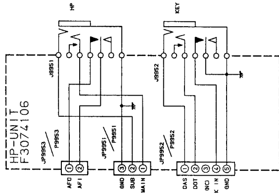
(HP Unit schematic diagram)
