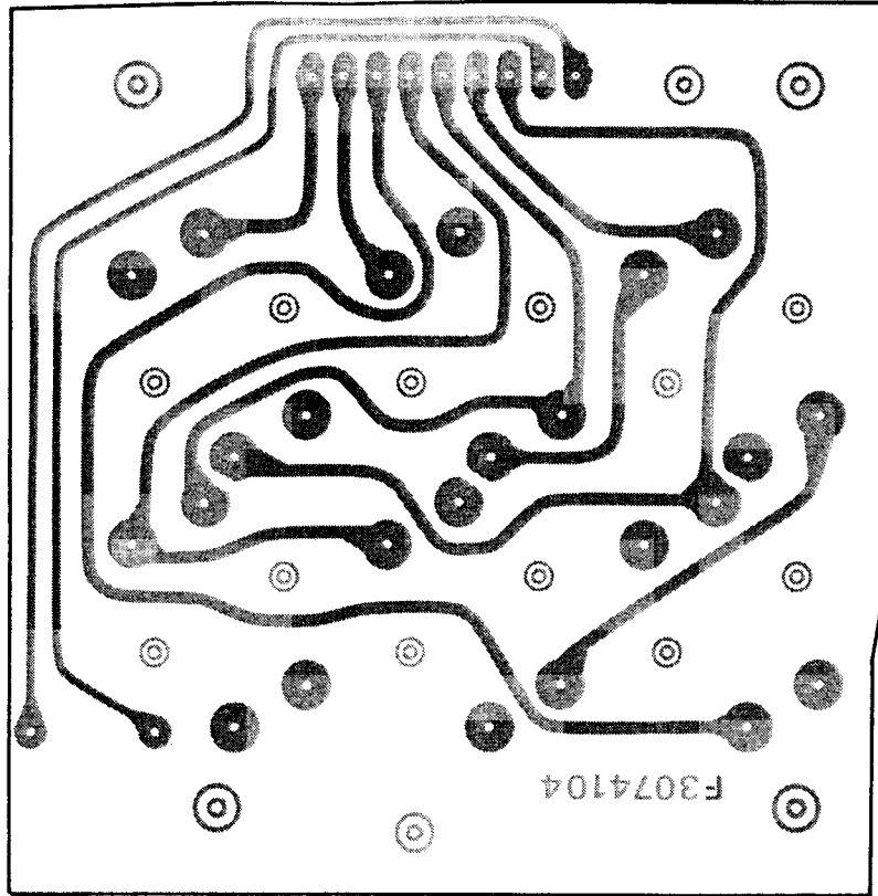
(obverse view of "solder" side)
