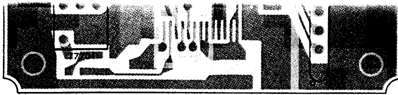
(obverse view of "component" side)
