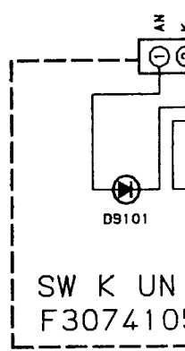
(SW K UNIT s
