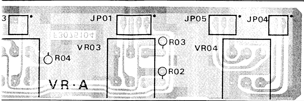
(obverse view of "component" side)
