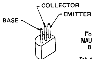
(obverse view of "solder" side)
