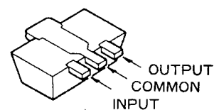
Marked Surface NJM78L05UA (05) (Q7703, Q7803)
