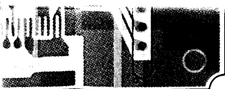
of "component" side)
