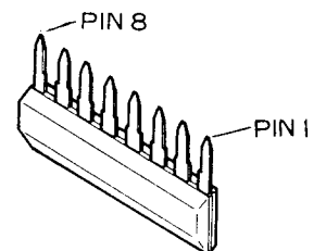
M5218L (Q7610, Q7611)
