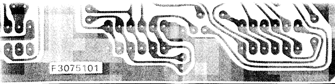
(obverse view of "solder" side)
