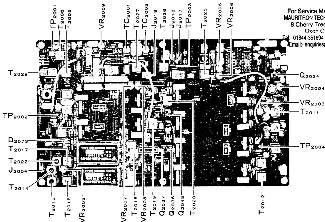
IF Unit: Receiver Test & Alignment Points
