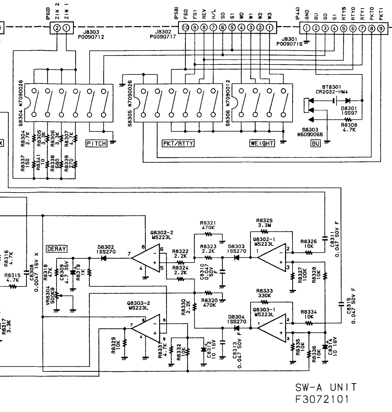
(schematic diagram)
