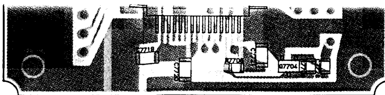
(obverse view of "chip-only" side)
