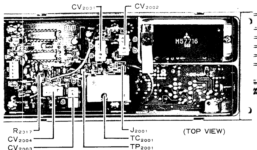
FEX-767-7 Alignment Points
