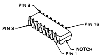
MC14028BCP (Q5006)
