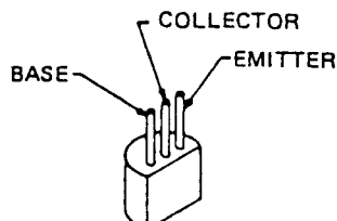
2SA684 (Q1009,1011,1012) 2SC945P (Q2009,2013) 2SC3354T (Q2007)
