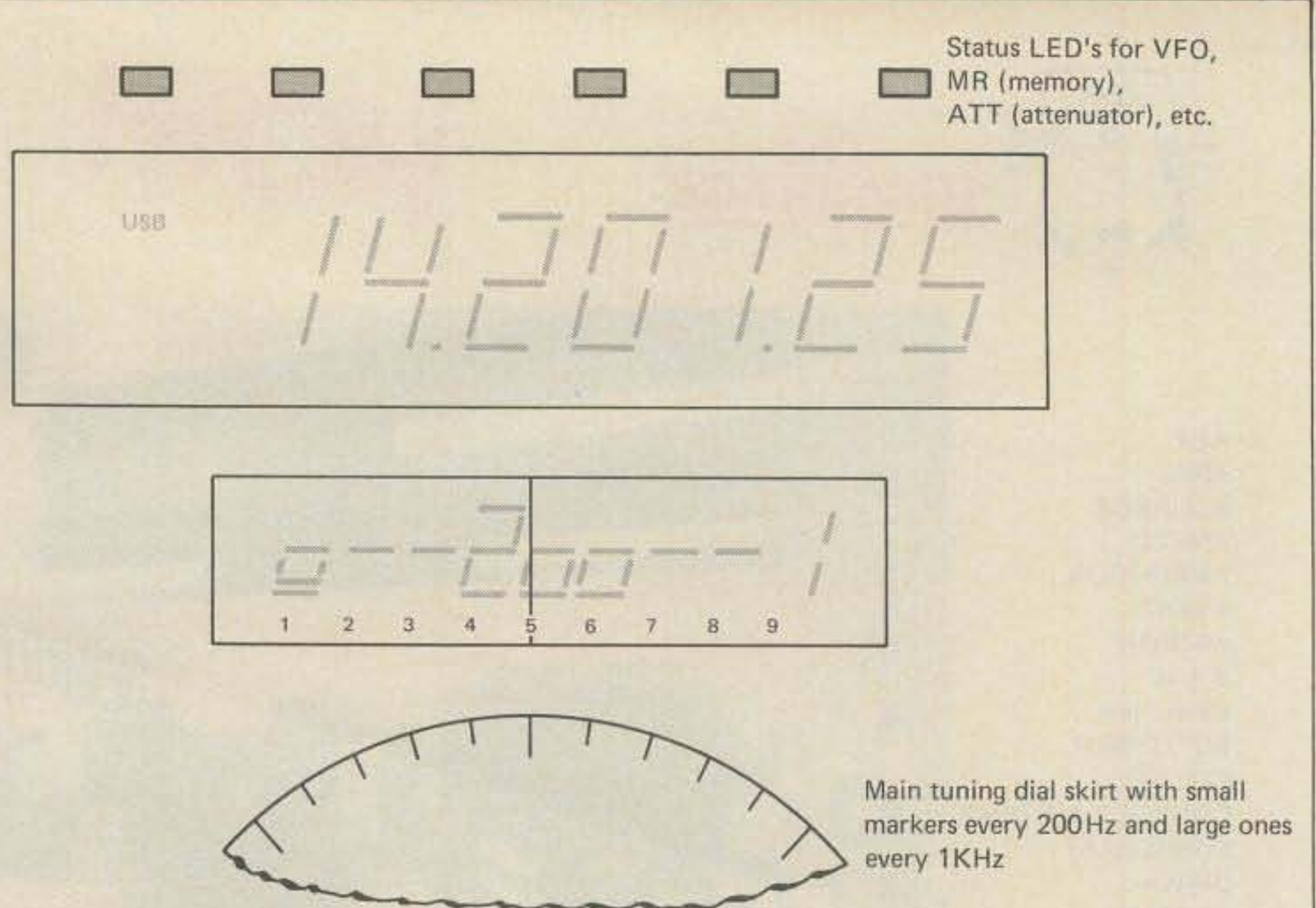
Fig. 6— An illustration and explanation of the digital frequency "scroll" feature in the FT-980.
