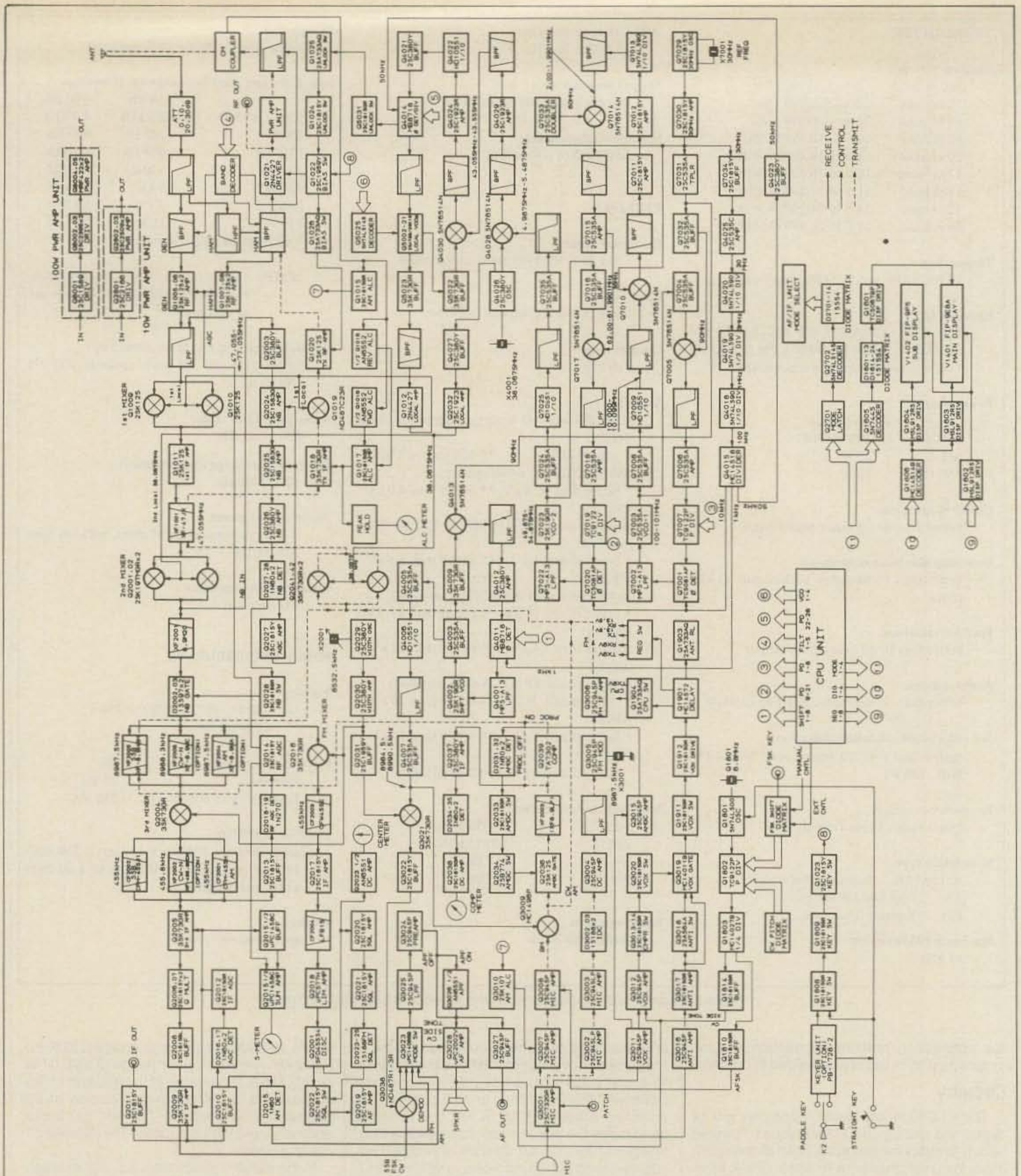
Fig. 1- Complete block diagram of the FT-980.
