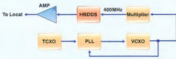
Local Oscillator block diagram
