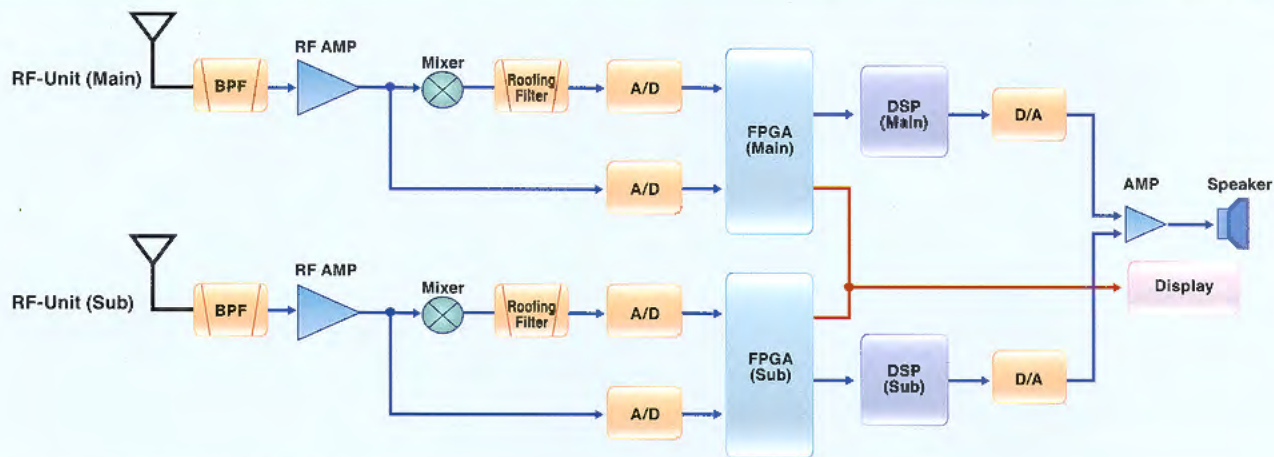
Completely Independent Dual Hybrid SDR System
