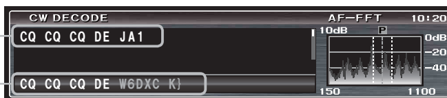
AF-FFT display (see page 40) ("Spectrum" or "Waterfall" display)
