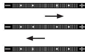
TUNING OFFSET INDICATOR
