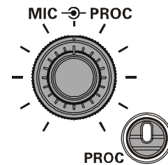
[MIC] knob / [PROC] knob
