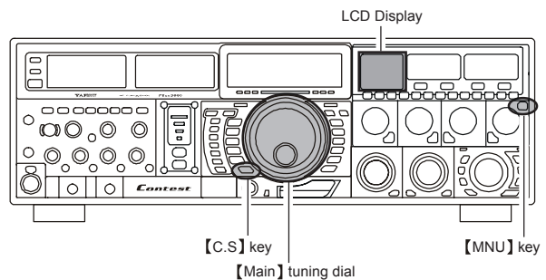
[Main] tuning dial
