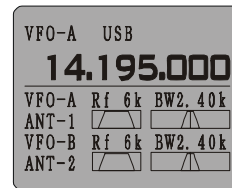
IF Shift system may be observed on the LCD
