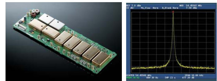
Local Oscillator Unit w/400 MHz HRDDS C/N Ratio Performance
