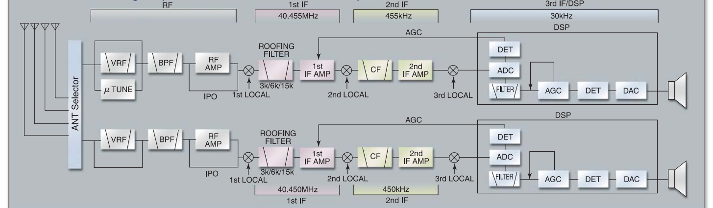
Three Selections of IF Roofing Filters 10 dB/Div · 200 kHz/Div
