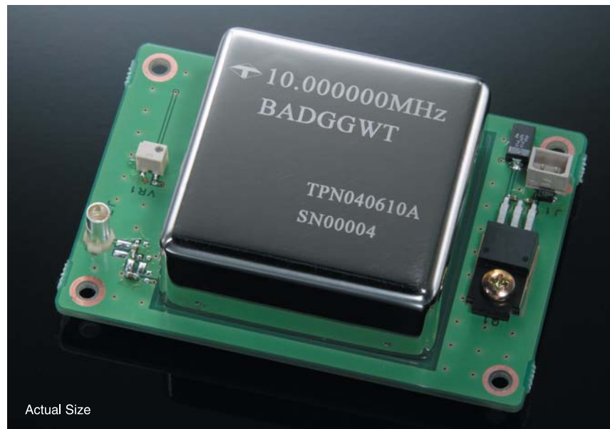
●2" x 2" (50 x 50 mm) OCXO Unit (Actual Size)
