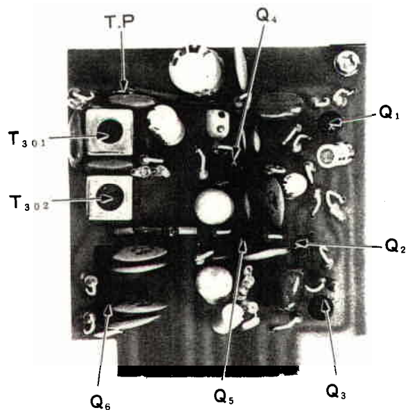
Fig. 22 FM UNIT
