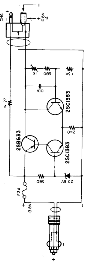
NC-8 * Adding resistor in parallel charges time constant
