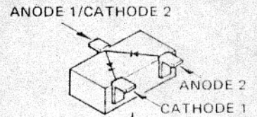
Marked Surface 1SS226 (C3) (D2013)
