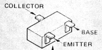
Marked Surface 2SA812 (M6/M7) (Q2015,2017,2020) 2SA1162GR (SG) (Q2019,2021) 2SC1623 (L6/L7) (Q2001,2003,2016, 2018,2022) 2SC2620B (QB) (Q2005,2010) 2SC2759 (U22) (Q2011,2012) 2SC3120 (HB) (Q2009)
