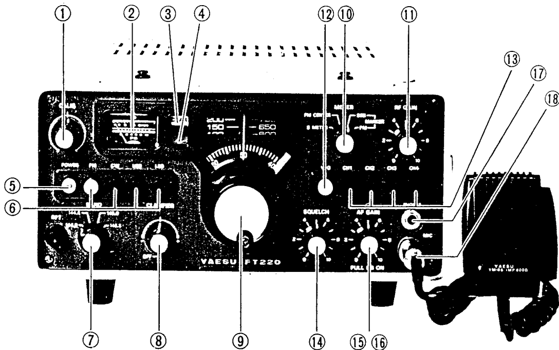
Figure 4 : Front Panel
