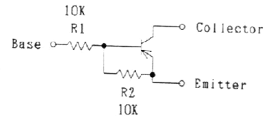
DTA114EK CIRCUIT DIAGRAM
