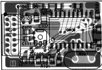
Obverse View of Chip Side
