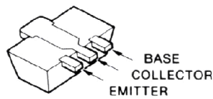
Marked Surface 2SB1301 (ZQ) (Q2010, Q2018)
