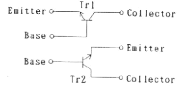
IMX3 CIRCUIT DIAGRAM
