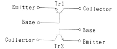
IMX1 CIRCUIT DIAGRAM
