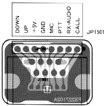
Obverse View of Connector Side
