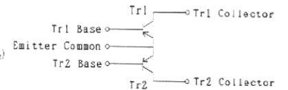
FMS1 CIRCUIT DIAGRAM
