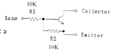
DTC114EK CIRCUIT DIAGRAM
