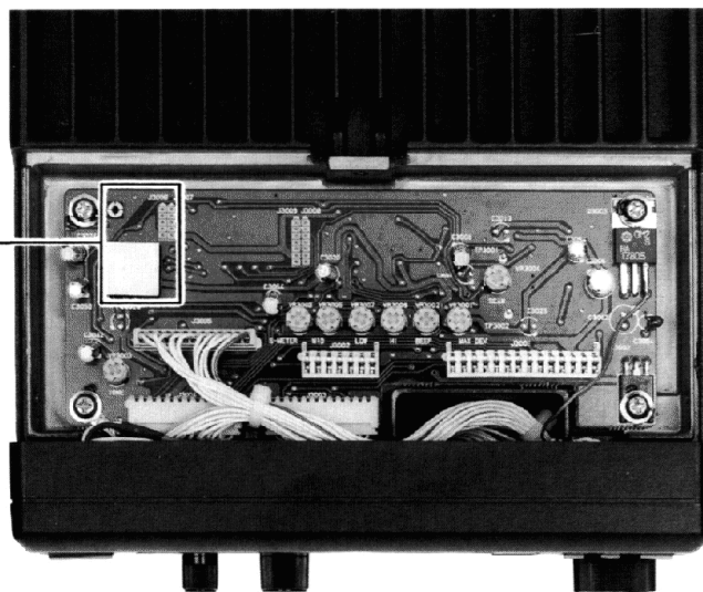
FTS-17A Mounting Location
