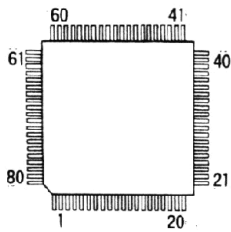
HD4074719H (Q2001)
