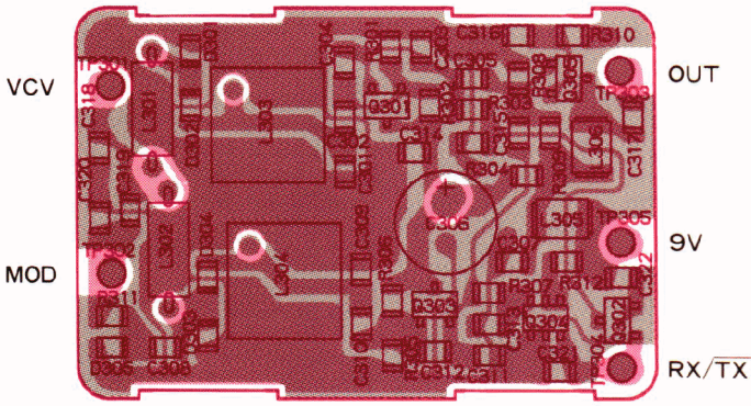
Obverse View of "Mixed Component" Side
