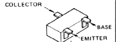
Marked Surface 2SA1162GR (SG) (Q2007) 2SC2712GR (LG) (Q2011) DTC144EK (26) (Q2005, Q2012)
