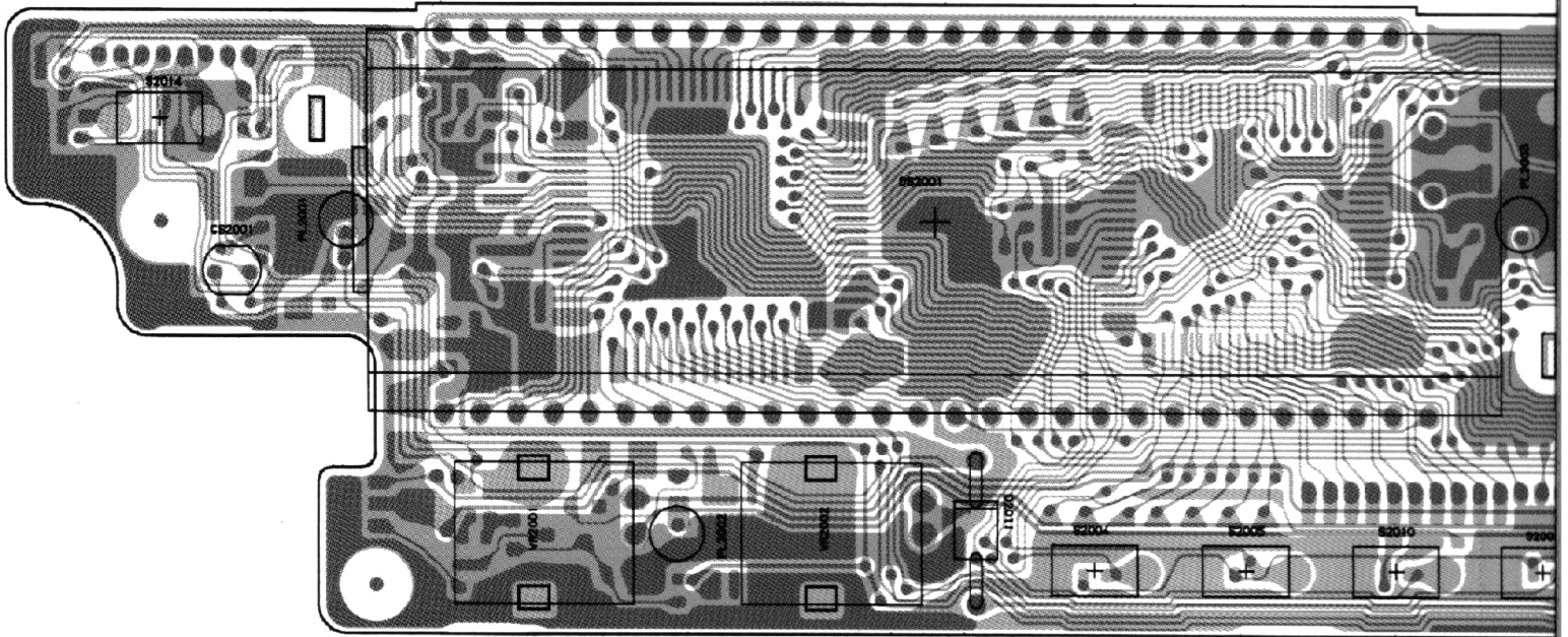
Obverse View of
