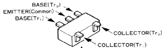
Marked Surface FMG4 (G4) (Q2015)
