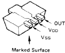
NJU7201 U50 (J1) (Q2003, Q2013) RH5VA45AA (D5) (Q2004)
