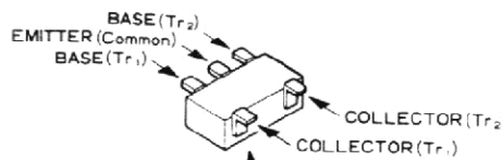
Marked Surface IMX1 (X1) (Q1018)
