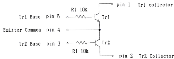
FMG4 CIRCUIT DIAGRAM
