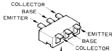
Marked Surface IMX1 (X1) (Q1018)
