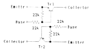
IMD2 CIRCUIT DIAGRAM
