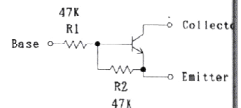
DTC144EK CIRCUIT DIAGRAM
