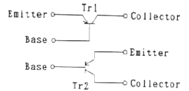
IMZ2 CIRCUIT DIAGRAM
