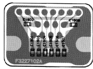
Obverse View of Chip Side
