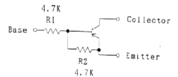
DTA143EK CIRCUIT DIAGRAM
