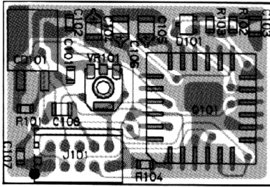
Obverse View of Chip Side
