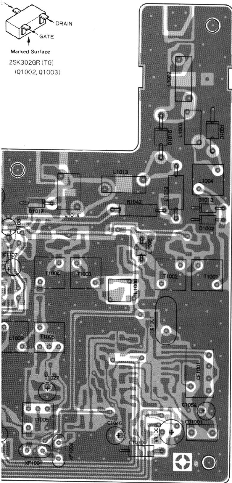
Obverse View of Leaded Component Side
