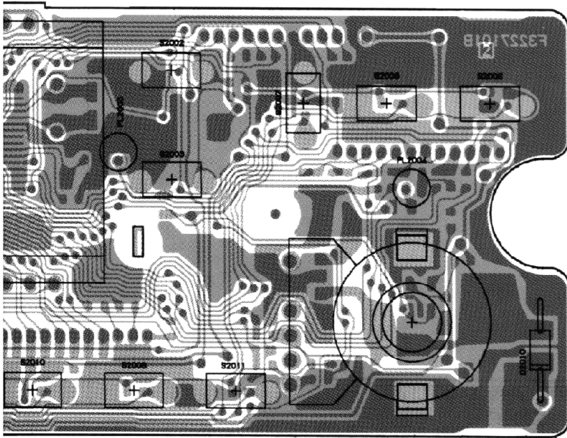
Reverse View of Leaded Component Side
