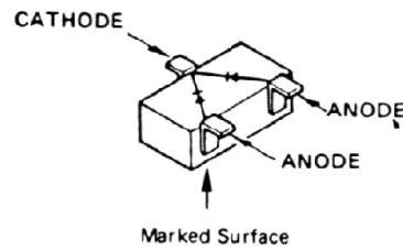
Marked Surface 1SS301 (B3) (D0101)
