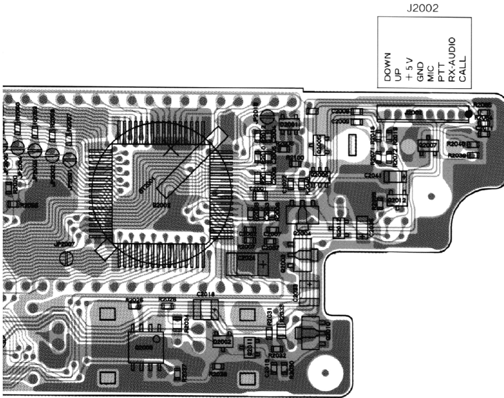
Obverse View of Chip Side
