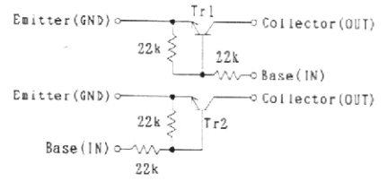
IMH5 CIRCUIT DIAGRAM
