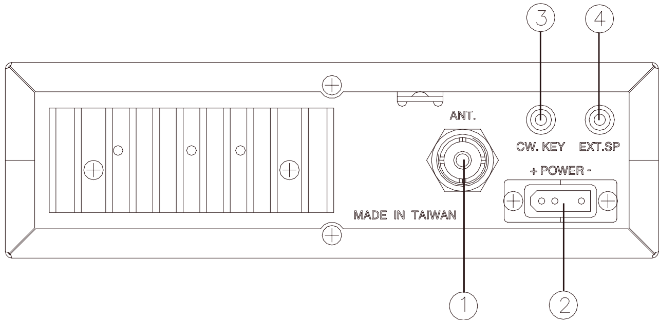
Figure 2-2 Rear Panel
