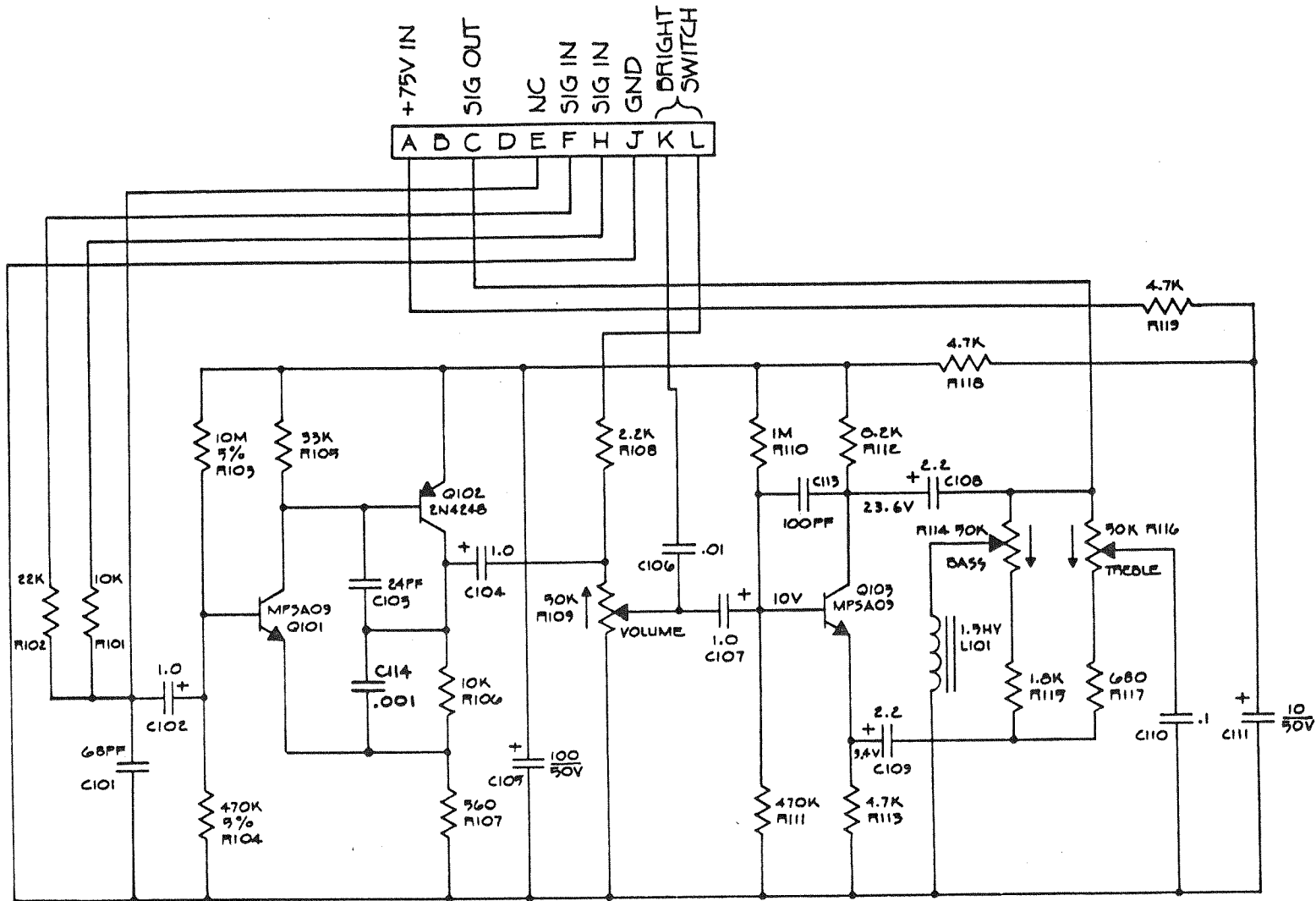
PREAMP (17-10)
