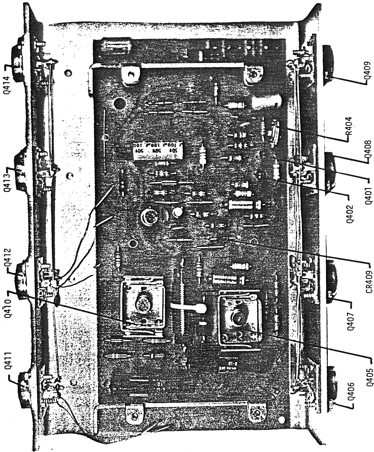
MODEL 270 - POWER AMP ASSEMBLY 843030 SCHEMATIC 1290D
