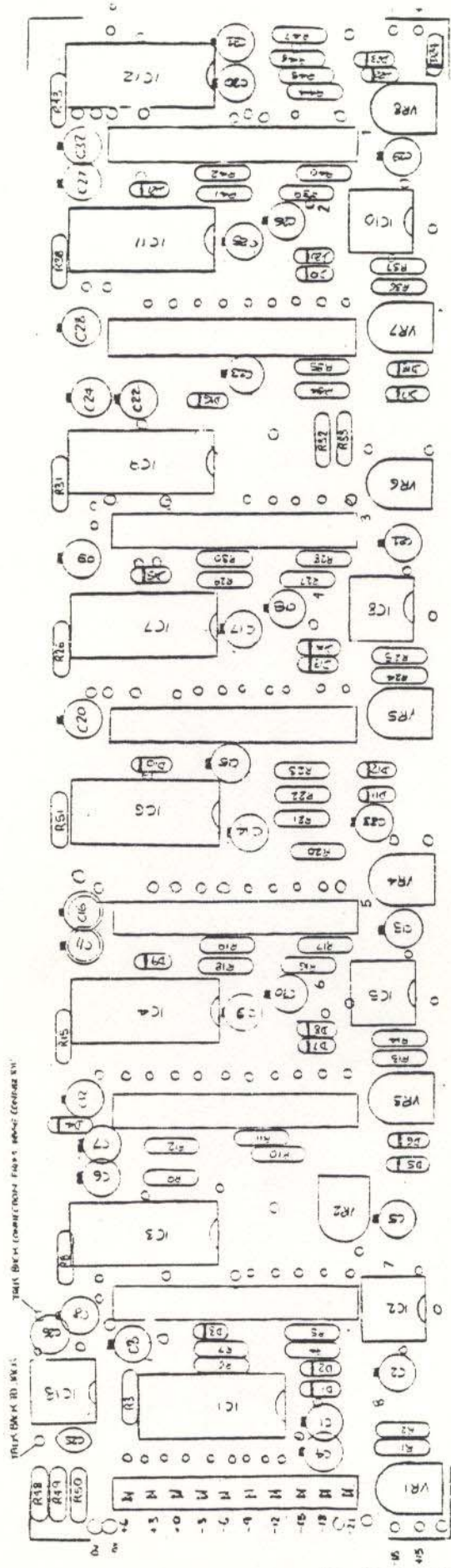
64106 METER POD PCB ISS 3 AGO109 AIB 69 SHIP DIRECT BRIGHTW
