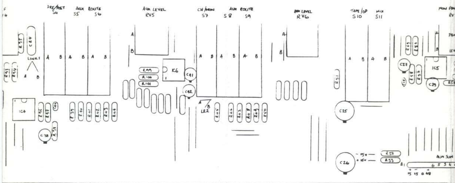
AHB CMC CHANNEL PCB COMPONENT OVERLAY 2:1
