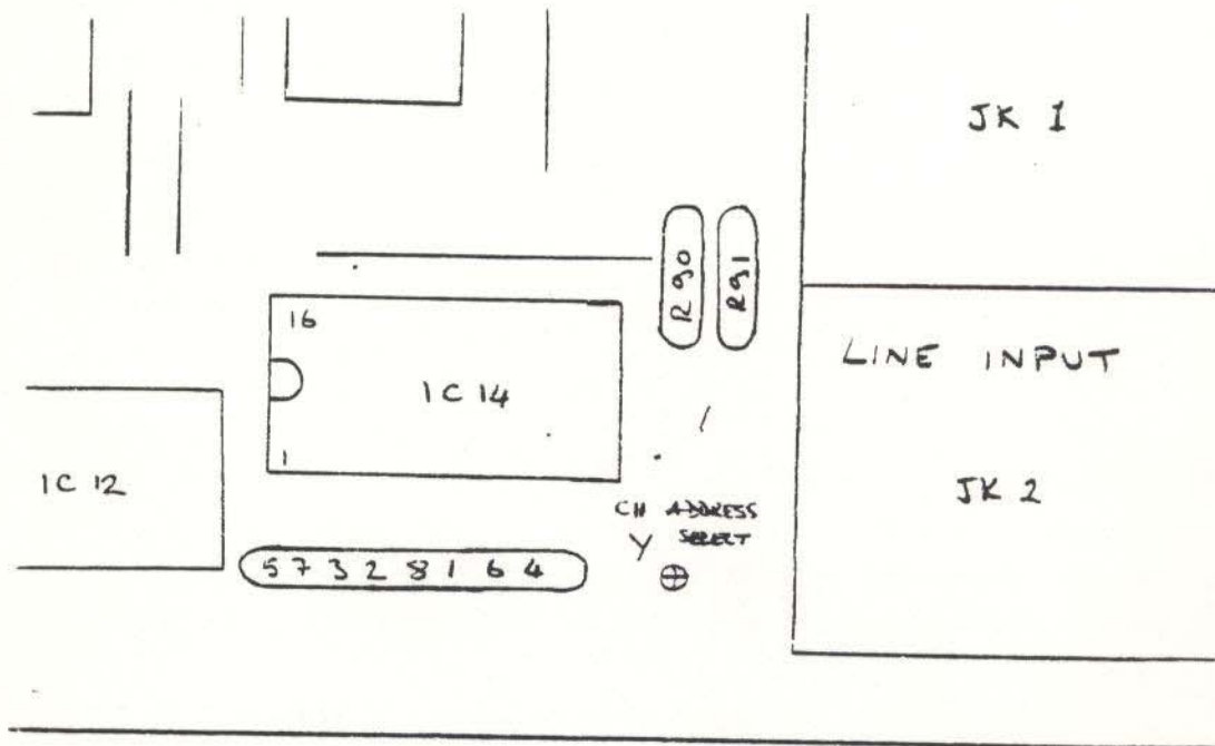
LINK Y LOCATION FOR CHANNEL P.C.B.
