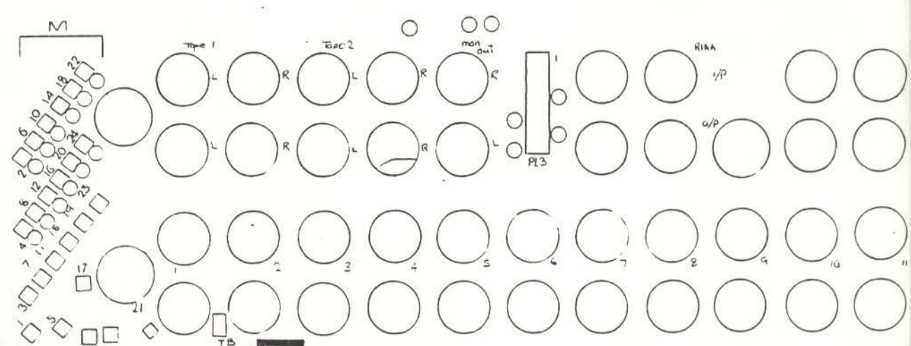
Mute + routing micro PCB layout p1
