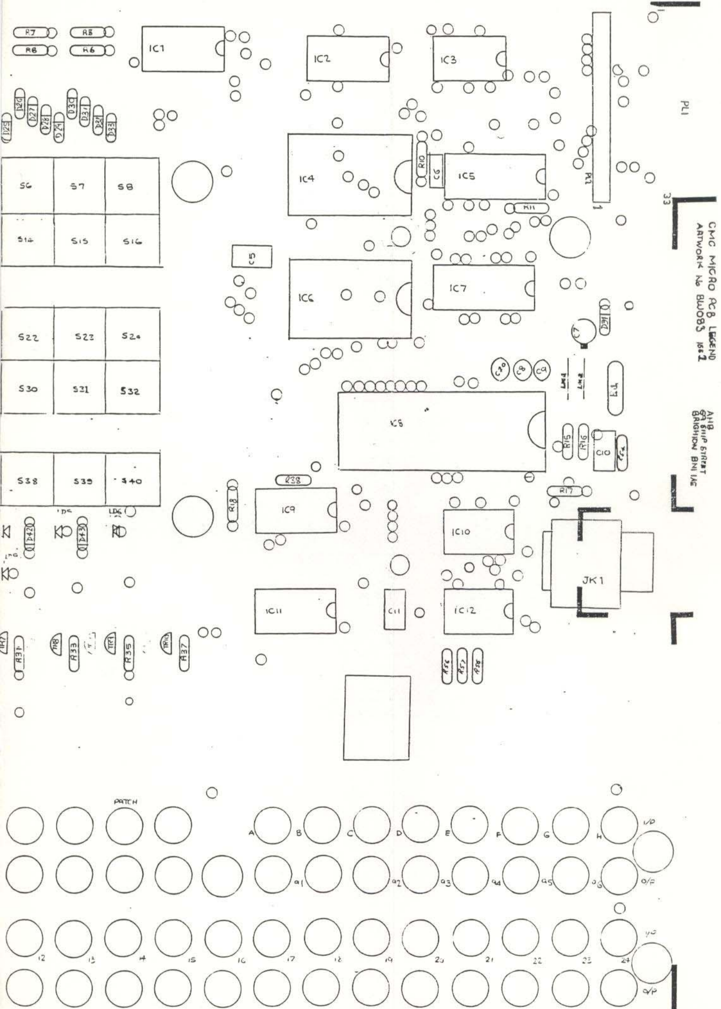
Mute + routing micro PCB layout p2
