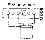
OUTPUT CONNECTIONS USING 15095 TRANSFORMER IN J5
