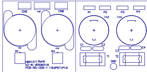
PCB:A2-IN TOP OVERLAY
