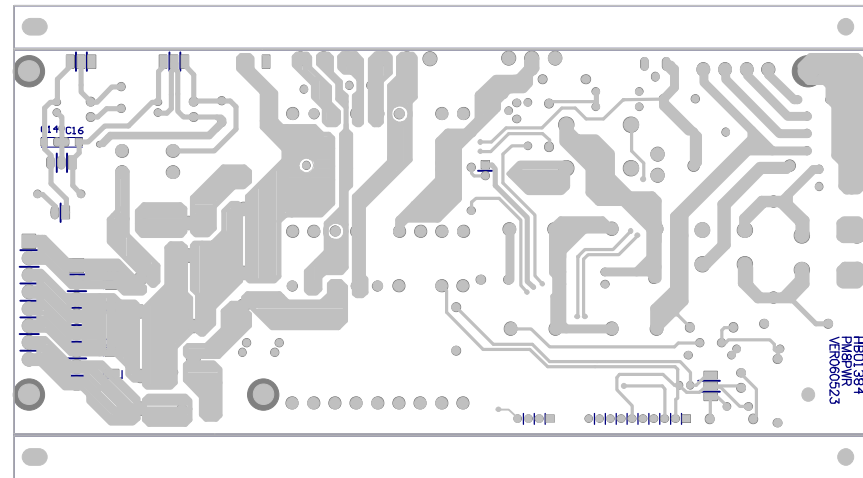
PCB:PM8PWR BOTTOM LAYER BOTTOM OVERLAY BOTTOM SOLDER
