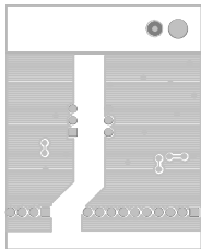
PCB:PM8CTL BOTTOM LAYER BOTTOM SOLDER
