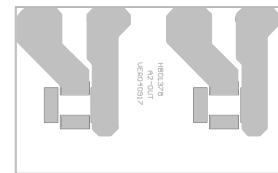
PCB:A2-OUT BOTTOM LAYER BOTTOM SOLDER
