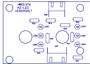
PCB:A2-LED TOP OVERLAY
