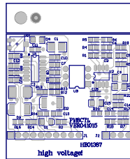
PCB:PM8CTL TOP LAYER TOP OVERLAY TOP SOLDER
