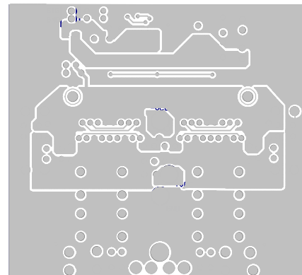
PCB:PM8PWR TOP LAYER TOP OVERLAY TOP SOLDER
