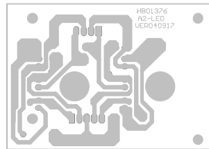
PCB:A2-LED BOTTOM LAYER BOTTOM SOLDER
