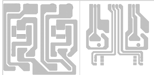
PCB:A2-IN BOTTOM LAYER BOTTOM SOLDER
