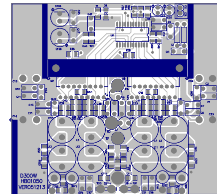
PCB:PM8PWR TOP LAYER TOP OVERLAY TOP SOLDER
