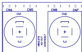
PCB:A2-OUT TOP OVERLAY
