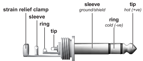
Fig. 4.5: 1/4" TRS connector
