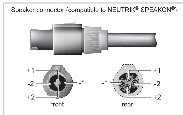
Fig. 4.1: Neutrik® Speakon®-compatible connectors
