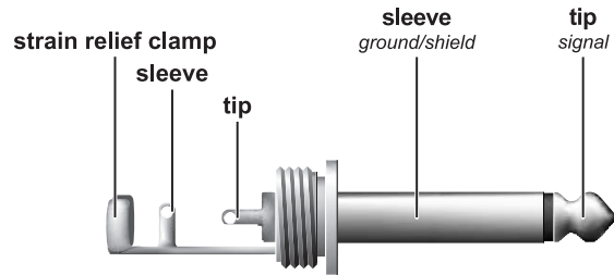
Fig. 4.4: 1/4" TS connector
