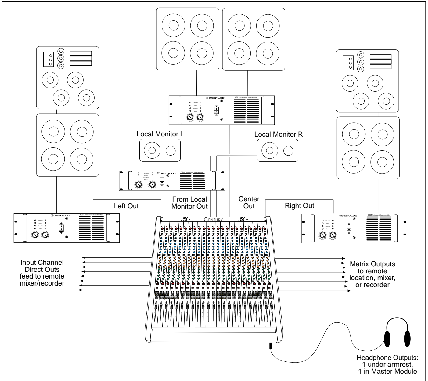
Output Connections
