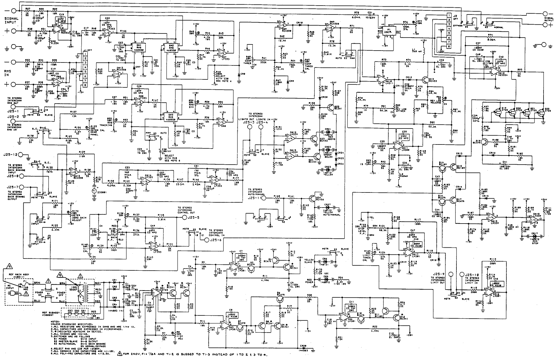
dbx® TITLE: SCHEMATIC 165A Compressor/Limiter 6110-00-01
