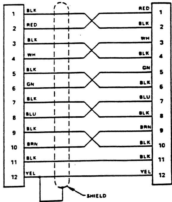
Fig. 7 - Stereo Coupler Cable
