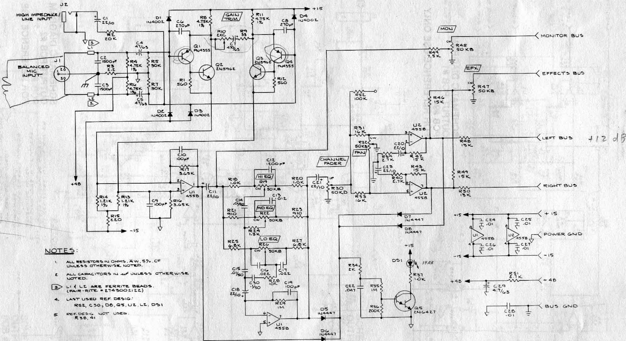
SCHEMATIC DIAGRAM INPUT PCB PCB #93 FOR REFERENCE USE ONLY
