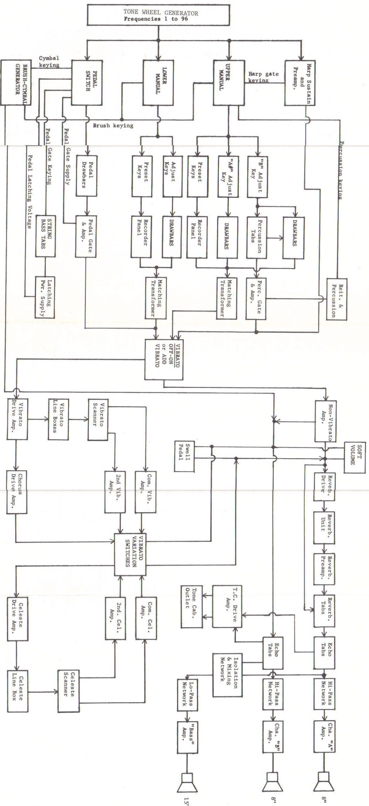
BLOCK DIAGRAM H-100 SERIES FIGURE 44
