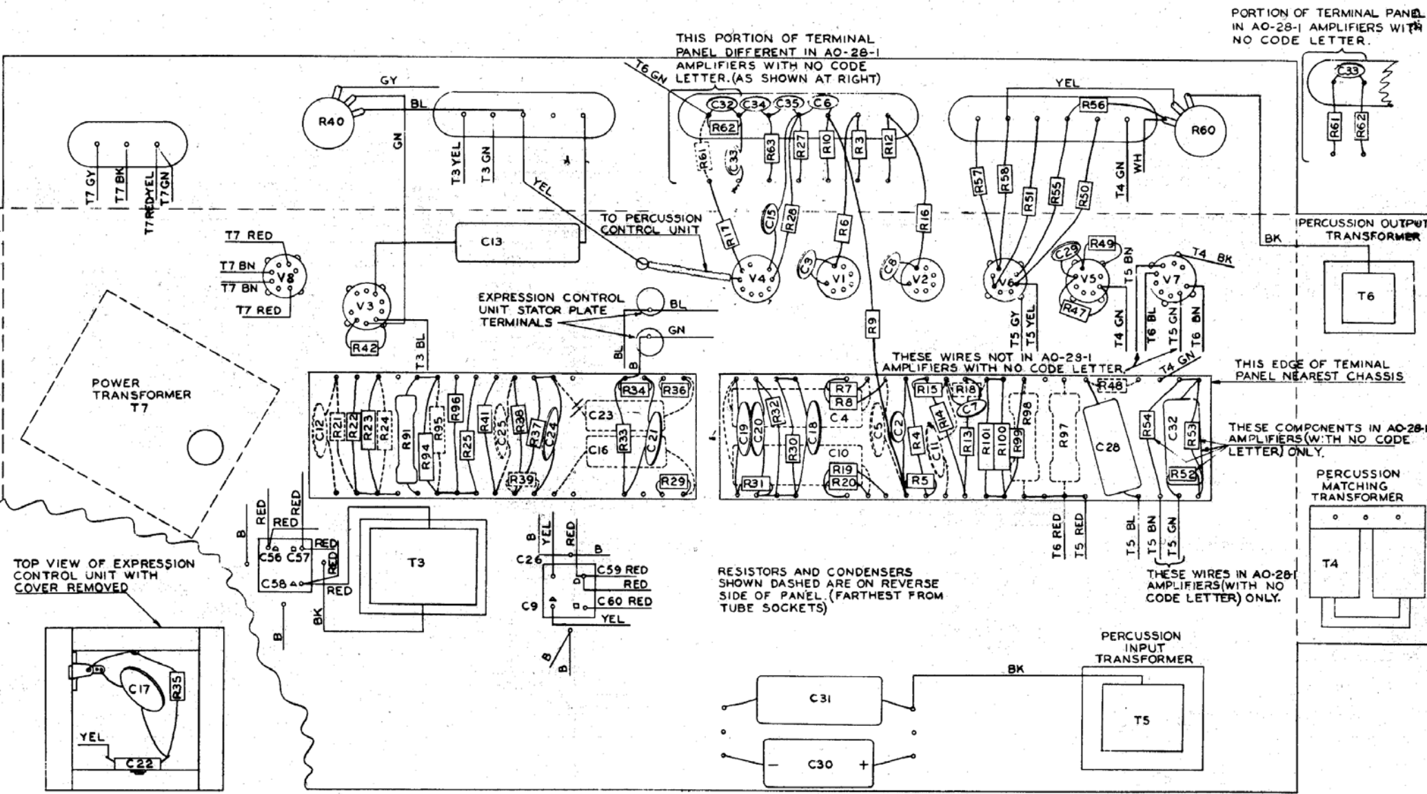
FIGURE 25-UNDERSIDE OF PREAMPLIFIER-TYPE AO-28 MODEL B3, C3, RT3 CONSOLES
