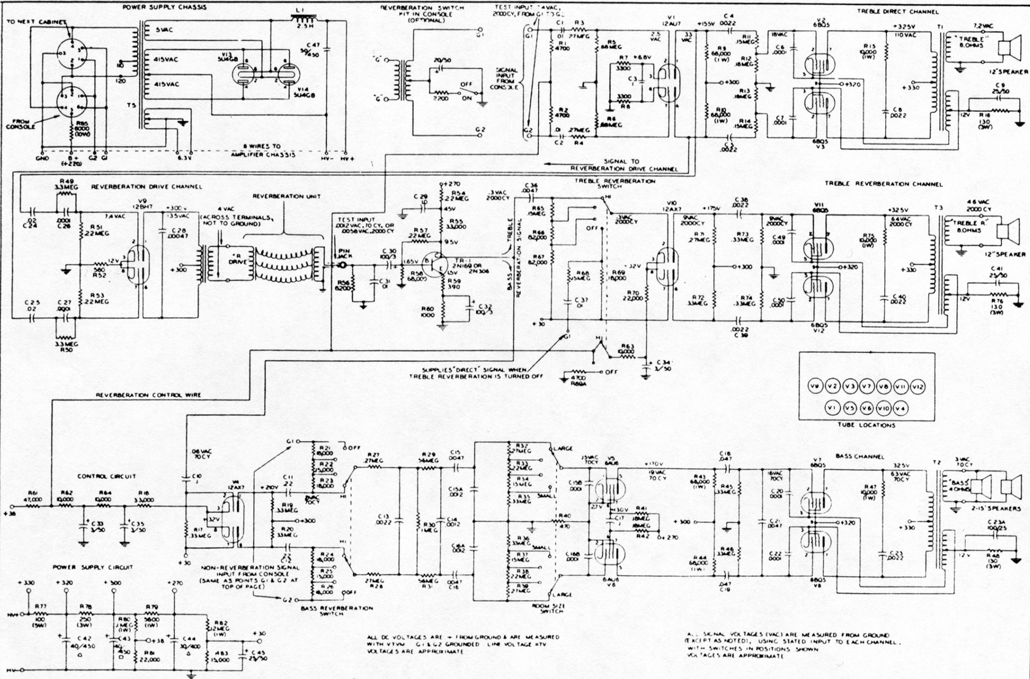
FIG. 26 AO-33-1 AMPLIFIER USED IN PR-40 AND OR-40 TONE CABINETS
