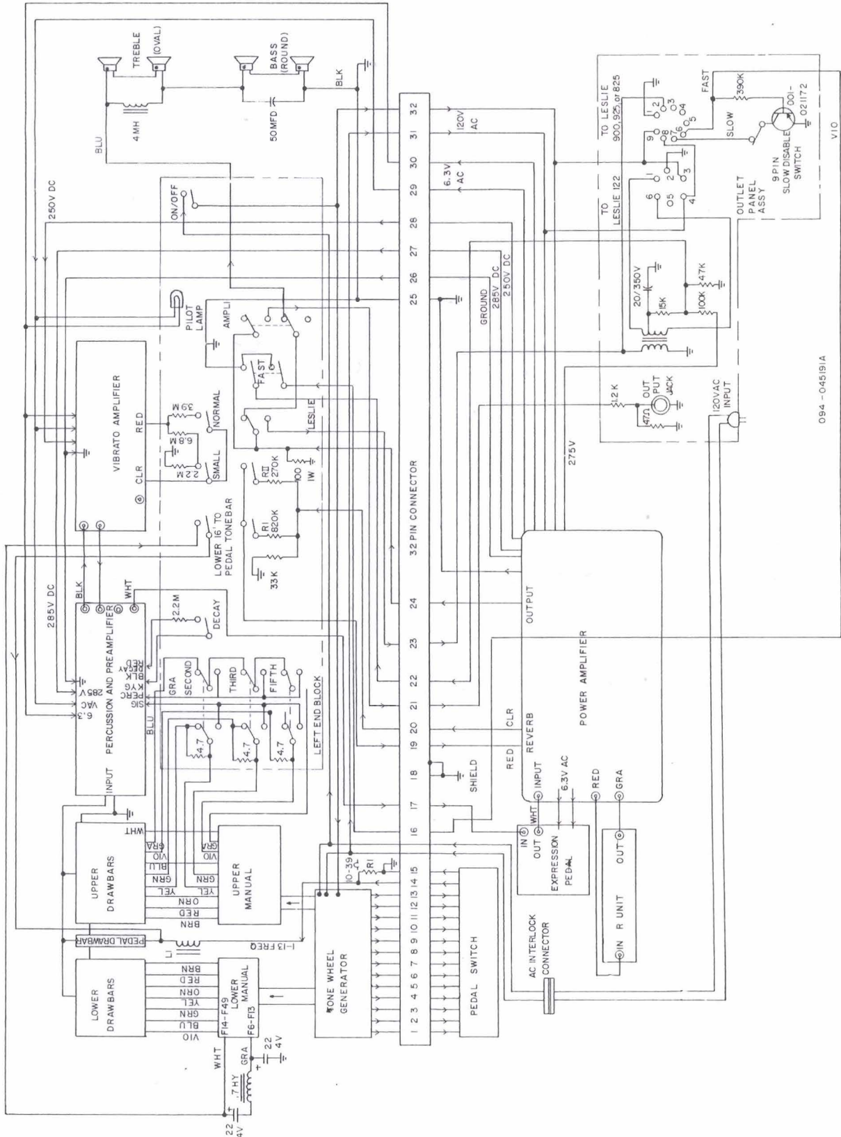
FIGURE 5-9 SYSTEM LOGIC DIAGRAM #2 (AFTER OCTOBER 15, 1971)
