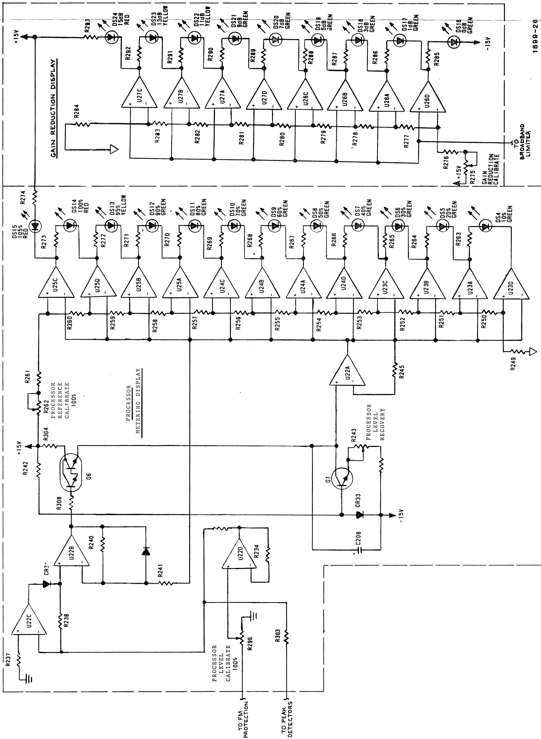
FIGURE 4-3. DETAILED BLOCK DIAGRAM FM LIMITER MODULE OUTPUT AND GAIN-REDUCTION METERING DISPLAY
