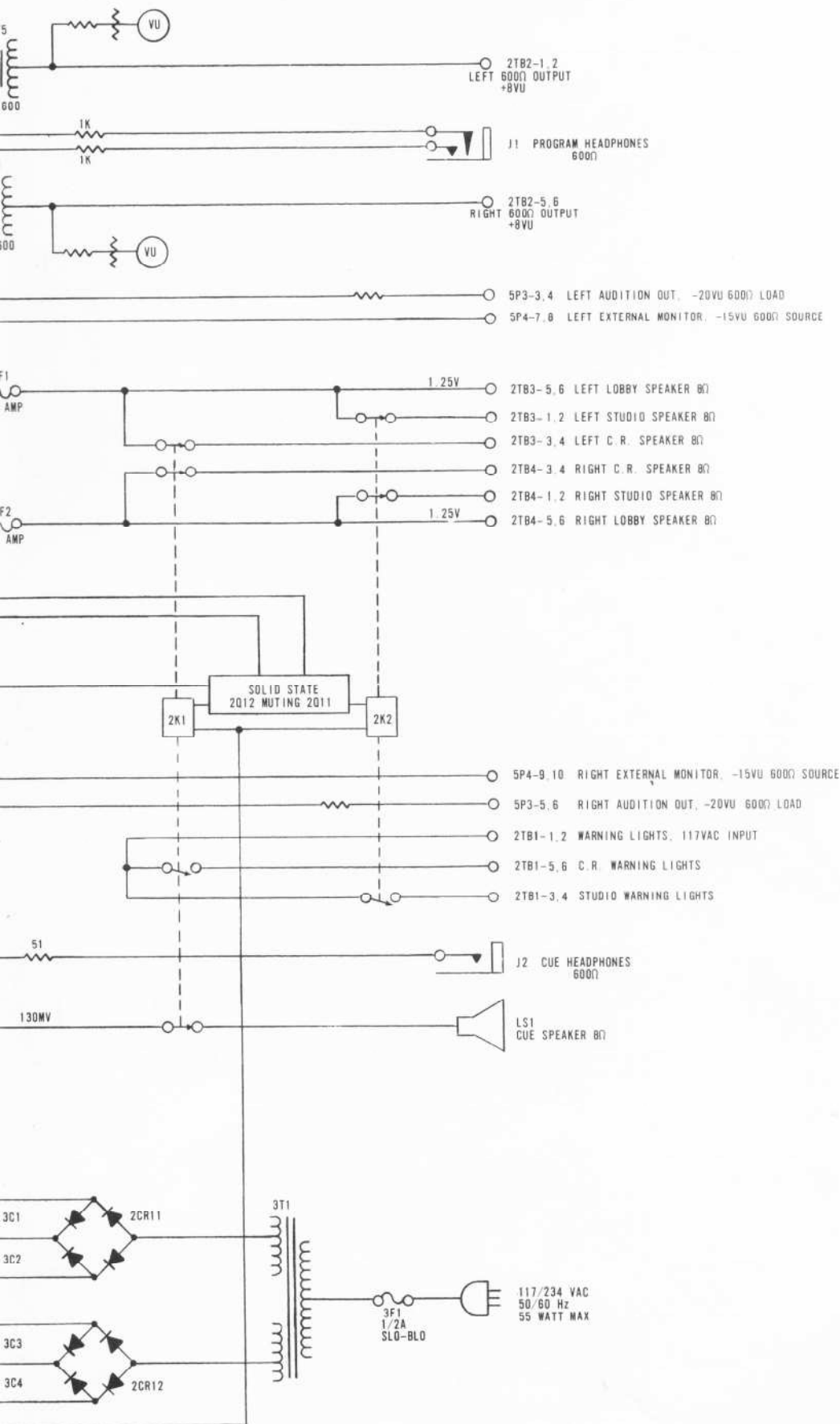
BLOCK DIAGRAM STEREO 5 CONSOLE 843 0721 001
