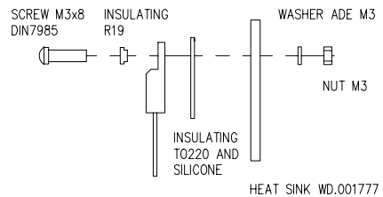
VOLTAGE REGULATOR ASSEMBLY DETAIL
