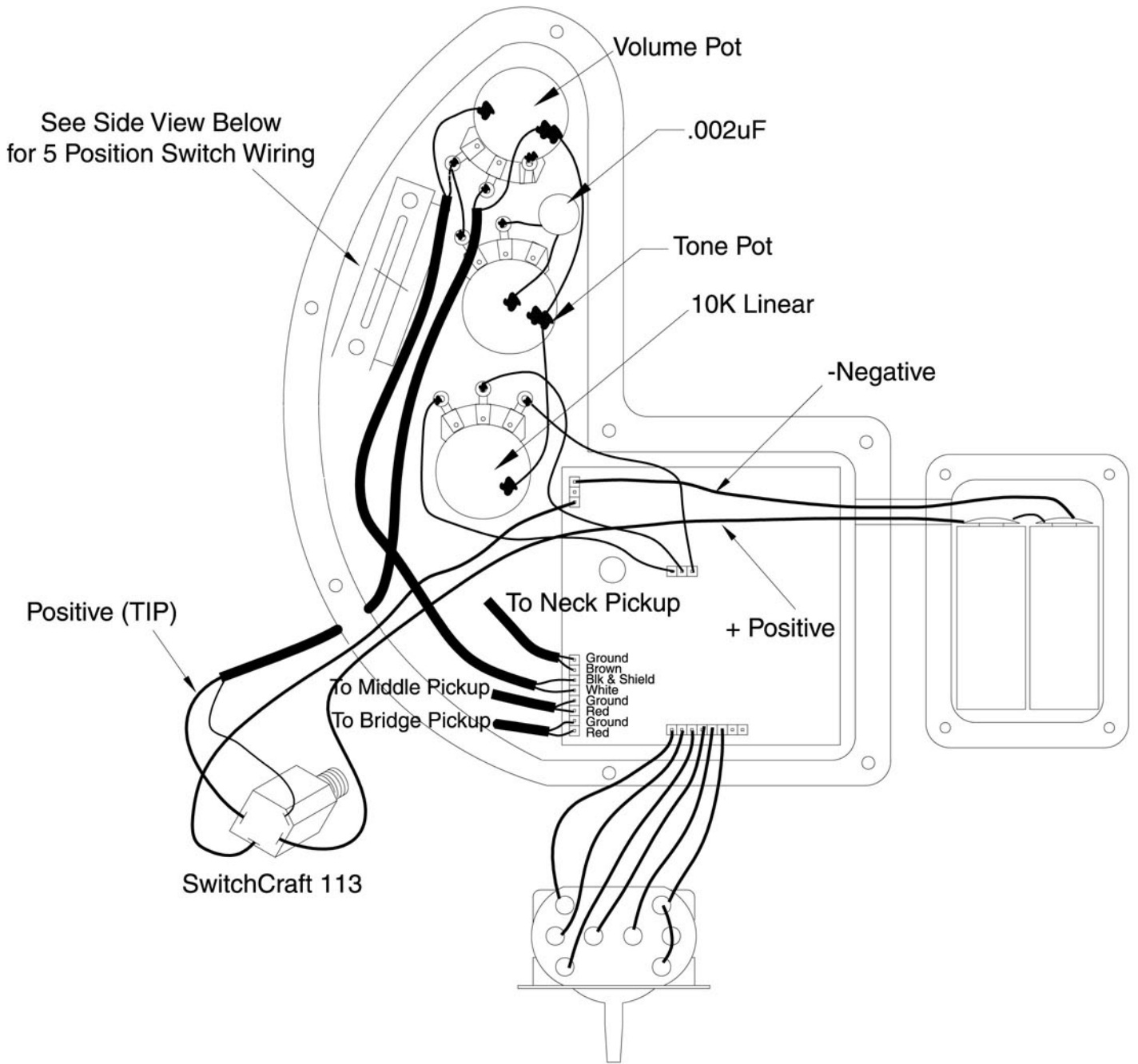
Kramer Sustainer Wiring Diagram
