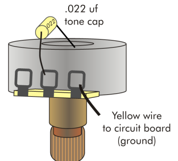
Tone pot wiring:
