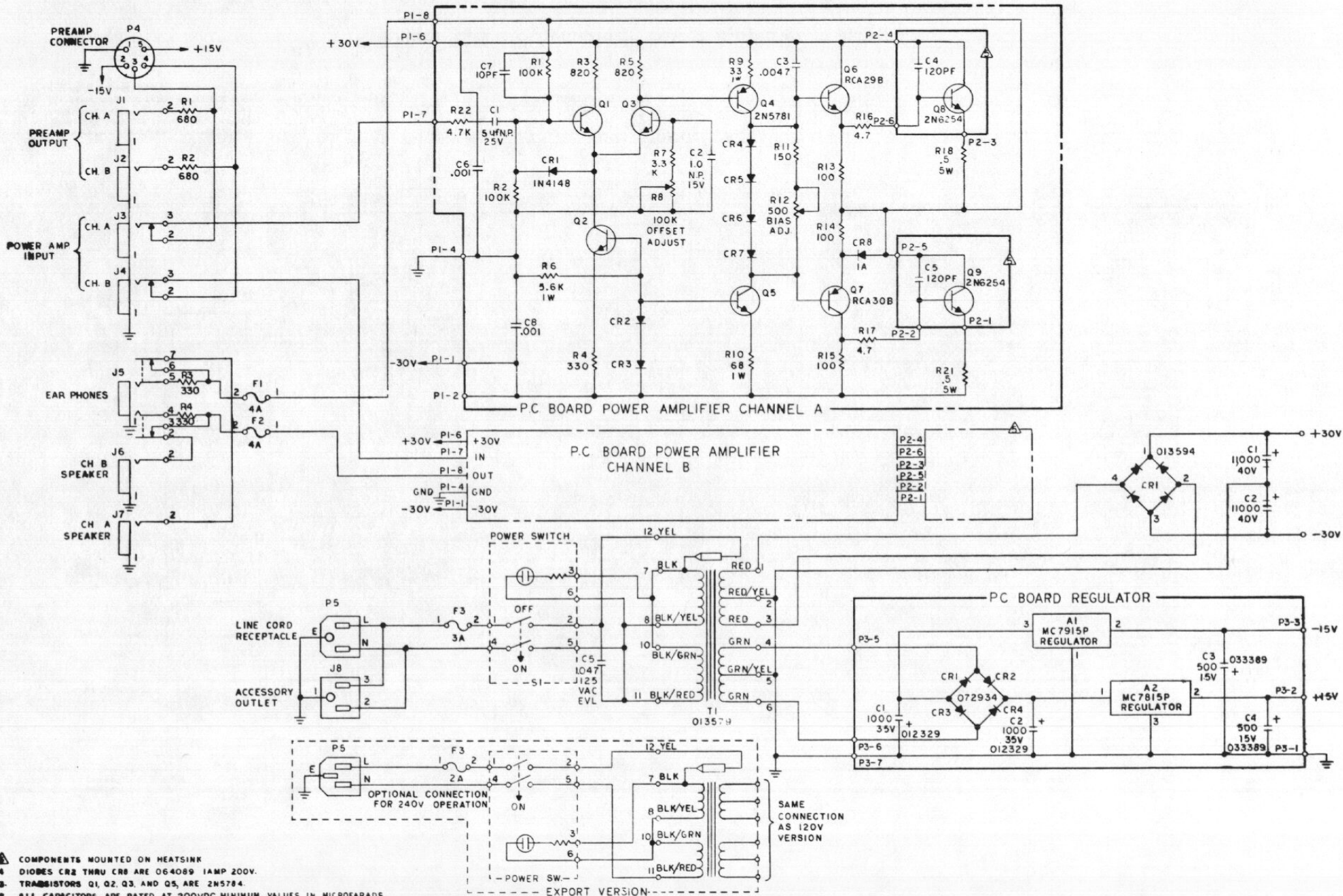
Figure 11-3. Schematic — Dual 50 Watt Power Amplifier — 100 Watt Suitcase and Janus I
