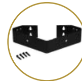
MTC-xxH* HORIZONTAL ARRAY BRACKETS
